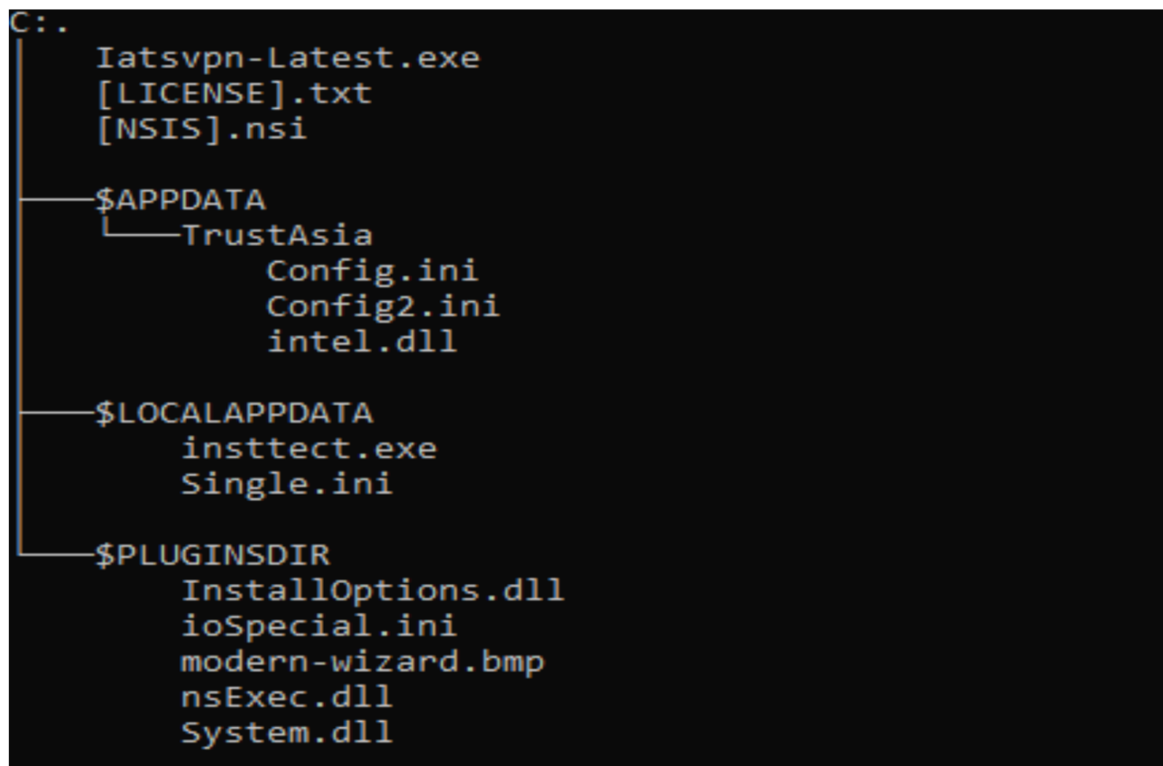
Figure 5: The extracted file structure by Lets.15.0.exe
