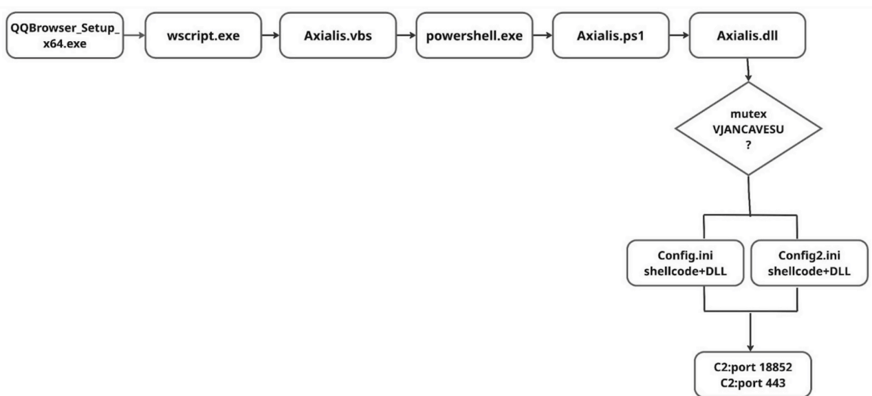
Figure 1: QQBrowser-Based Infection Flow Observed in MDR Case
