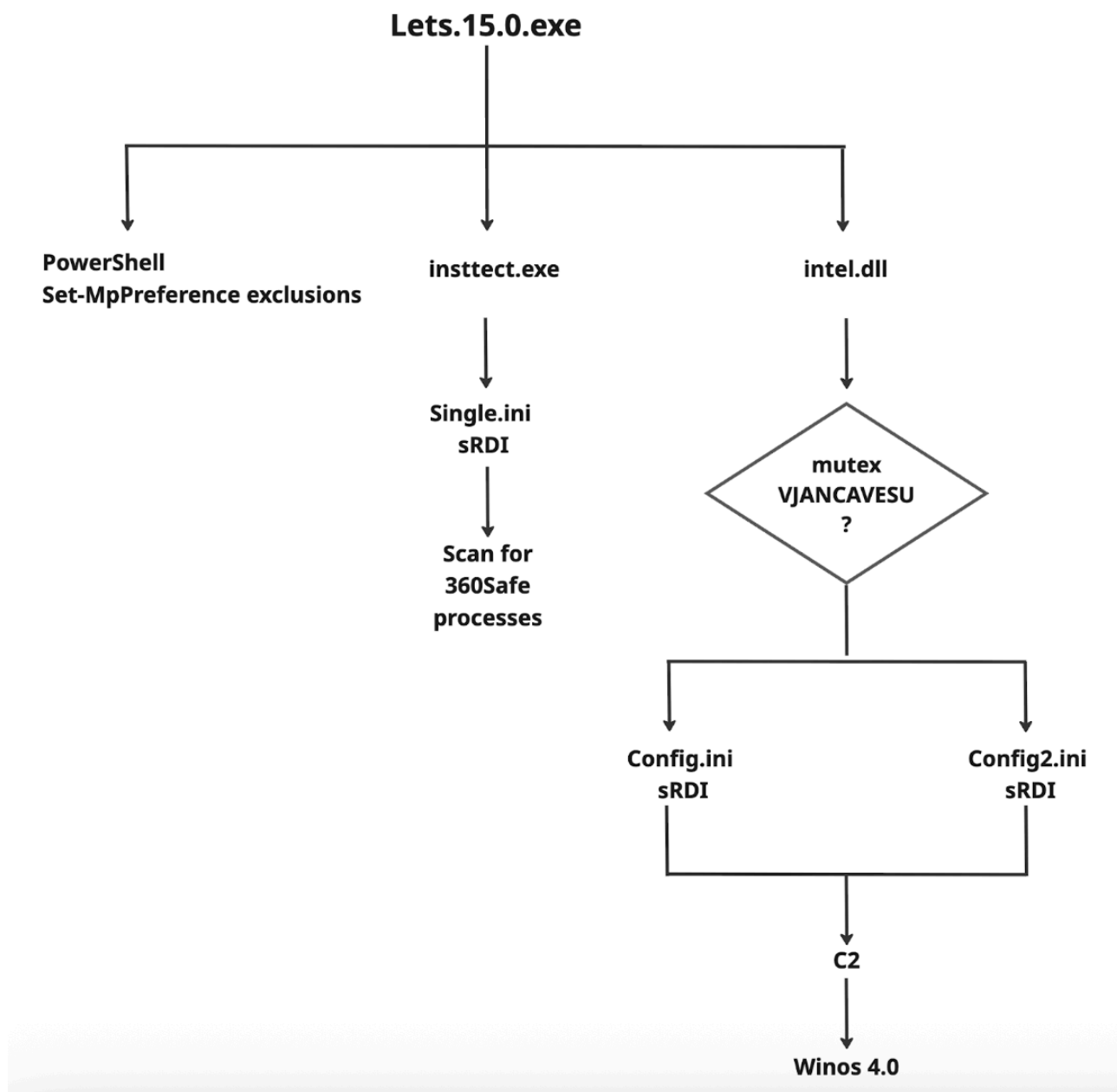
Figure 4 Catena Loader: From LetsVPN Installer to Winos v4.0
