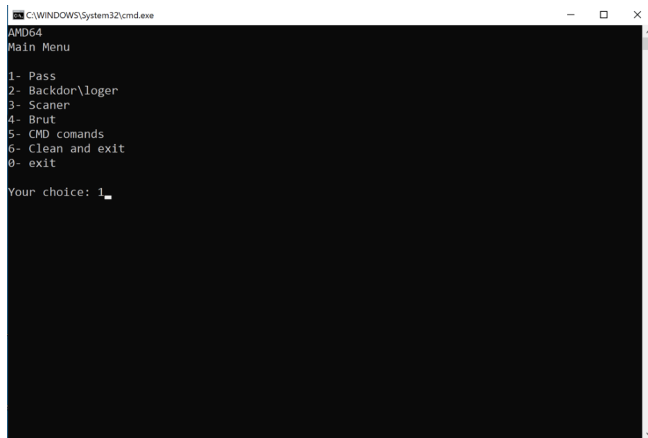
Figure 1. Overview of main menu options, as seen in the menu.bat execution
