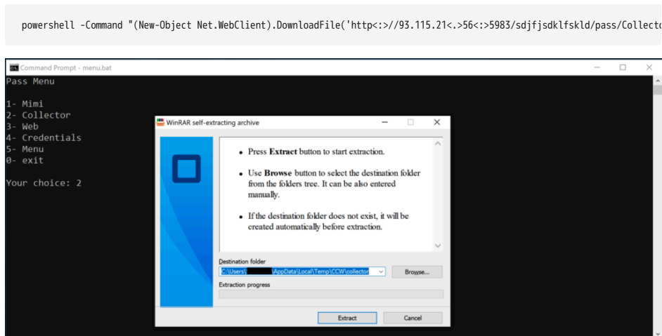
Figure 3. The attacker protects downloaded tooling through WinRAR self-extracting password-protected archives
