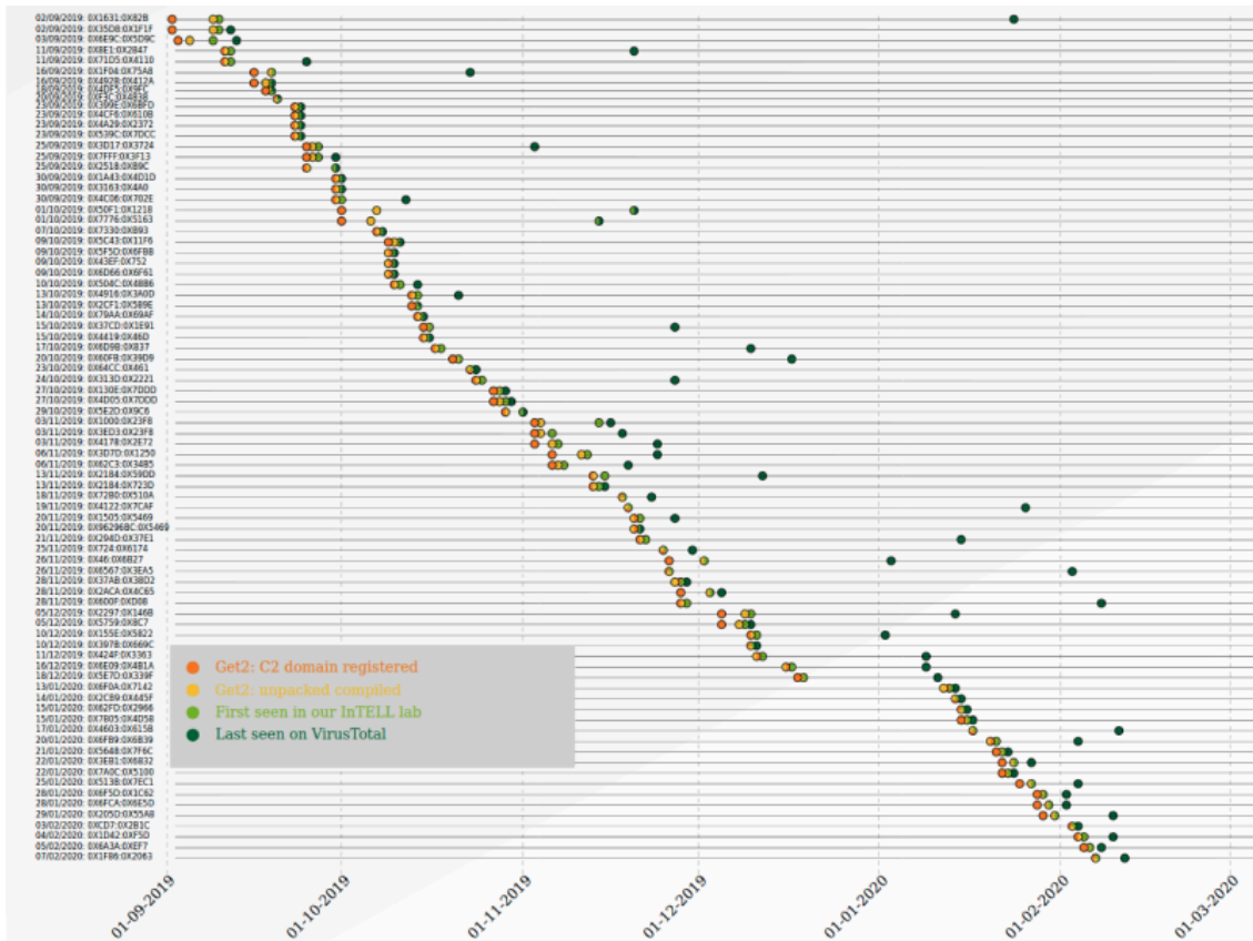
Figure 5. Dataset 1, Campaigns overview
