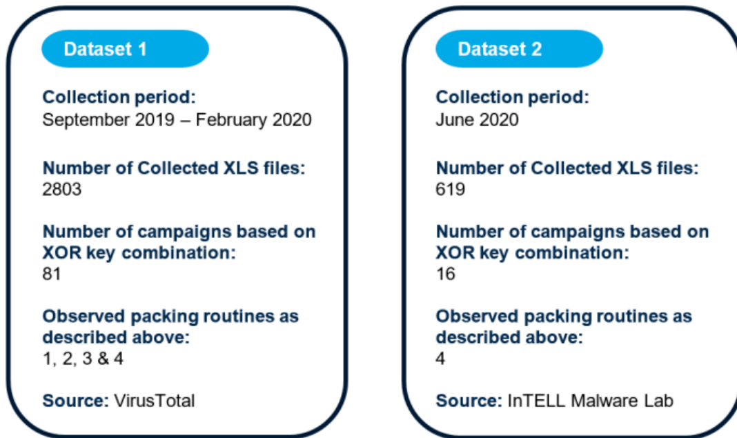
Figure 4. Datasets Statistics
