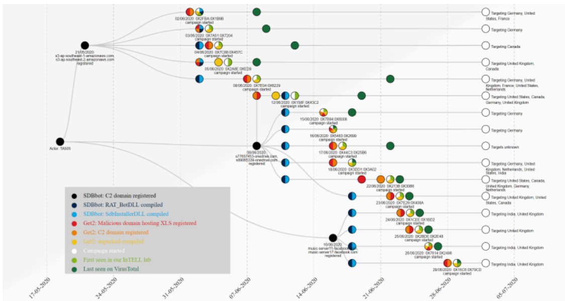
Figure 7. Dataset 2, Campaigns overview
