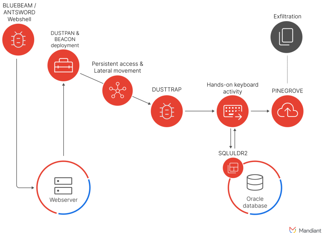
Figure 1: Attack path diagram of observed APT41 attack
