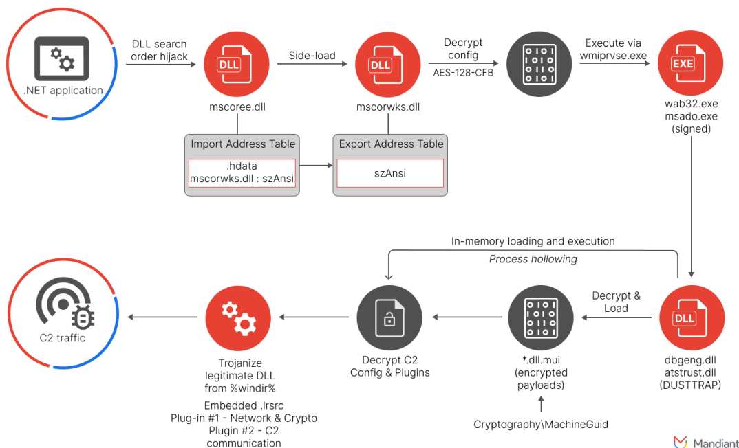
Figure 3: Full execution flow of DUSTTRAP
