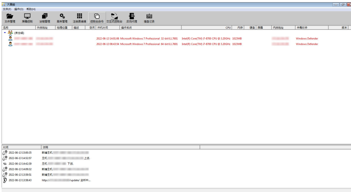
Figure 6. Connection established
