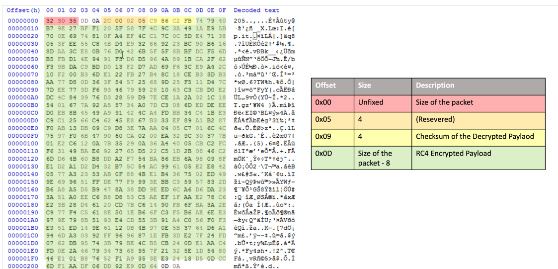
Figure 8. Encrypted information of the compromised machine
