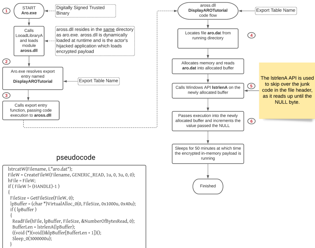
Figure 4. DLL sideloading overview for Aro.dat
