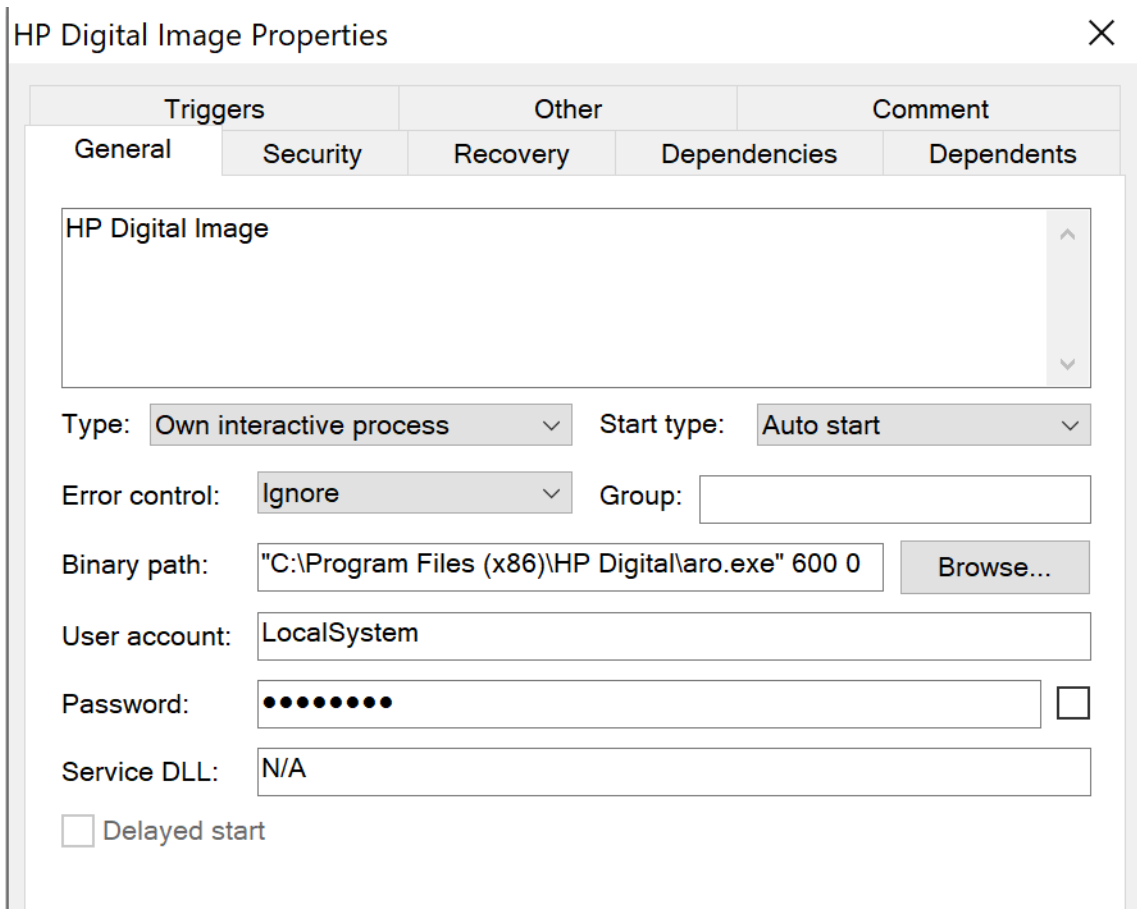
Figure 9. PlugX sample running as HP Digital Image
