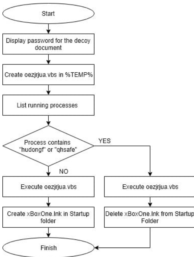
Figure 3 : Behaviour of VBScript in the HTML file
