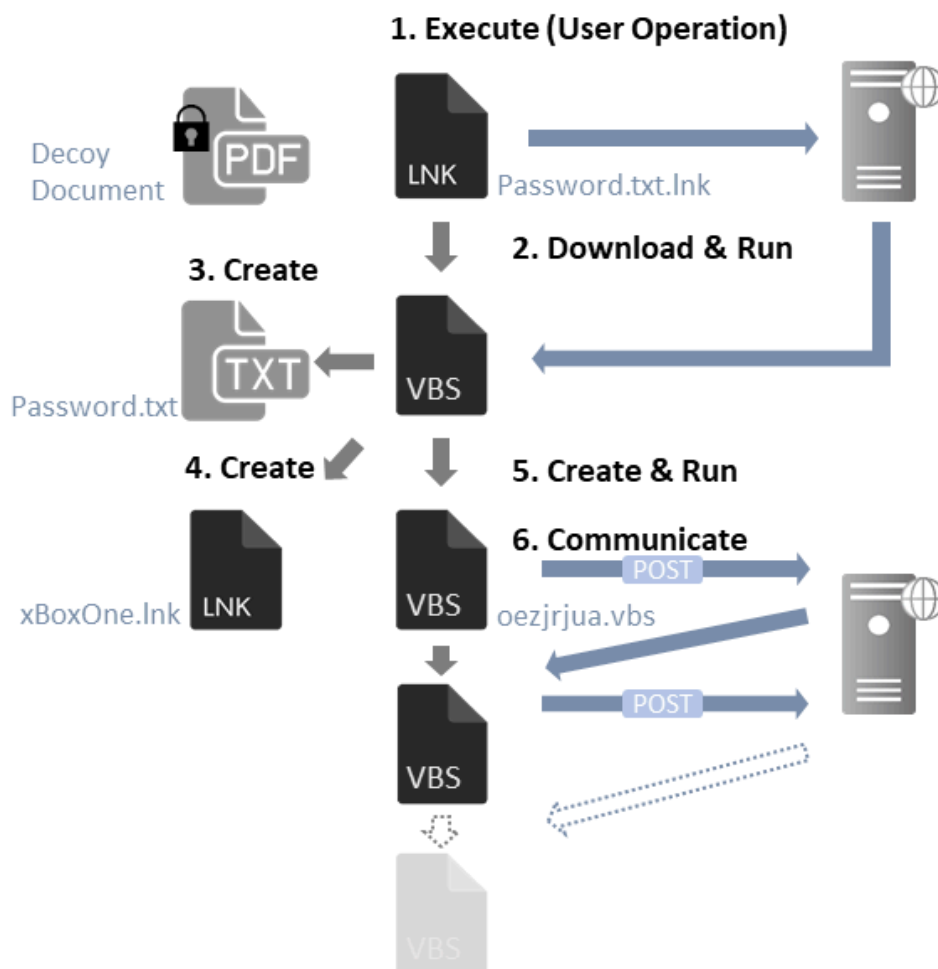
Figure 1 : Flow of events from running the shortcut file to infecting a host
