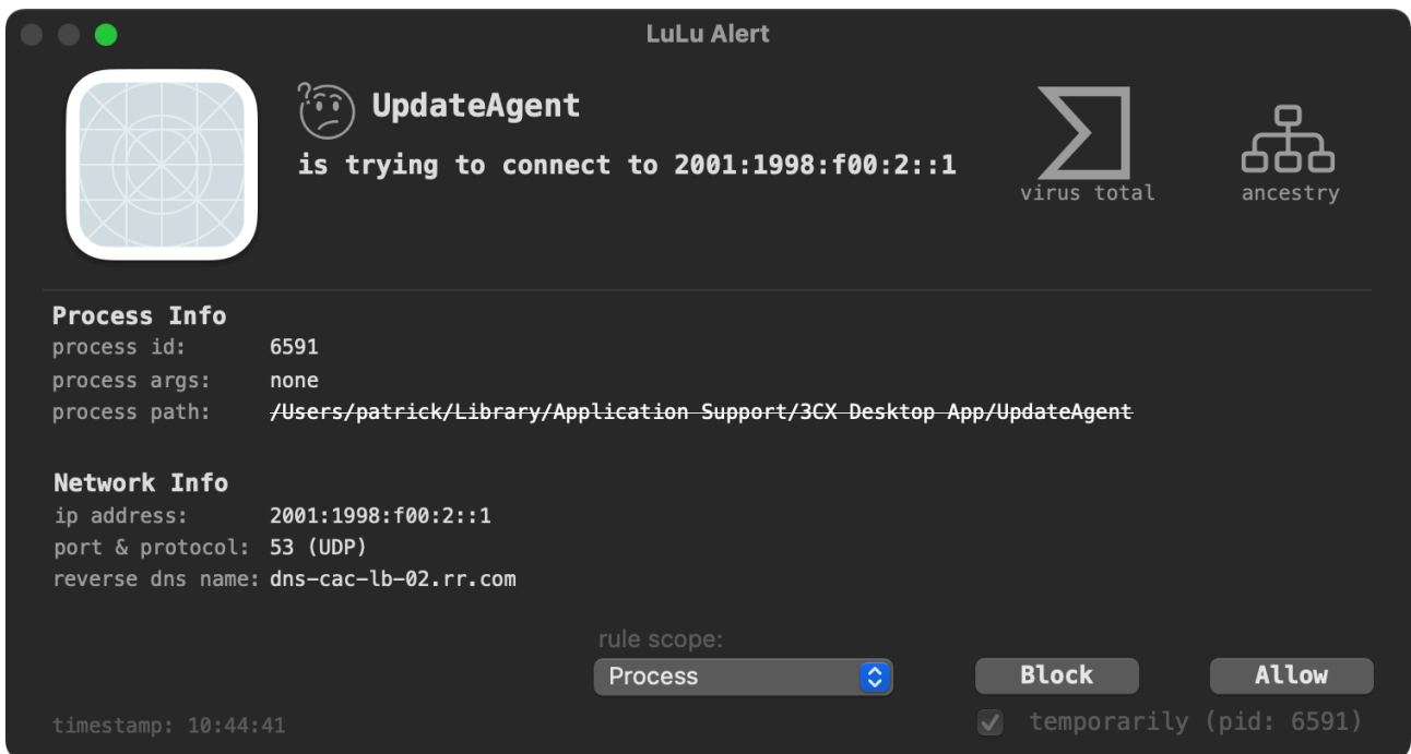
LuLu ...detecting unauthorized network access
