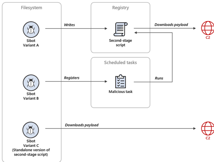
Figure 10. Sibot variants
