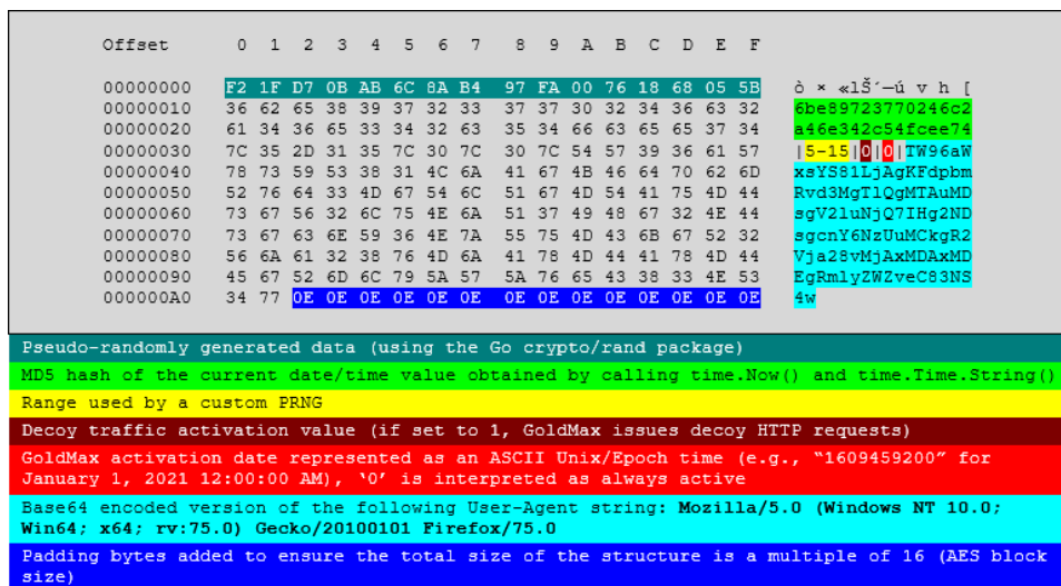
Figure 2. Data structure of the GoldMax configuration data
