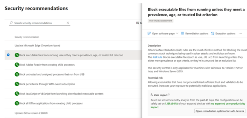
Figure 13. Security recommendations in threat and vulnerability management
