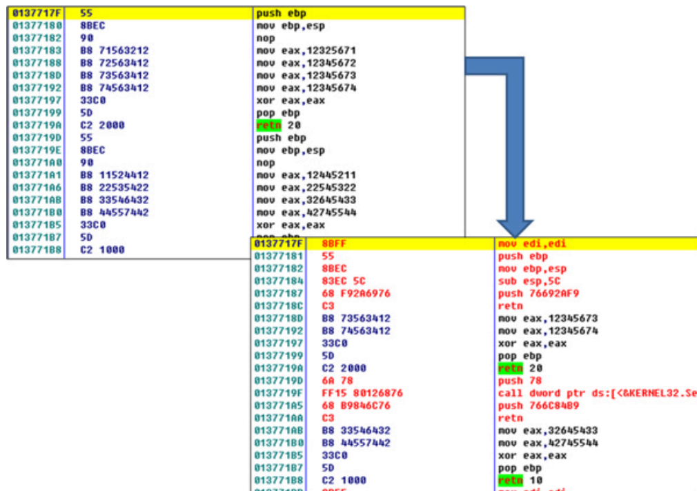
Figure 8. Pre-defined location used to store dummy code, now stores the initial instructions (in red) and a jump to the API.
