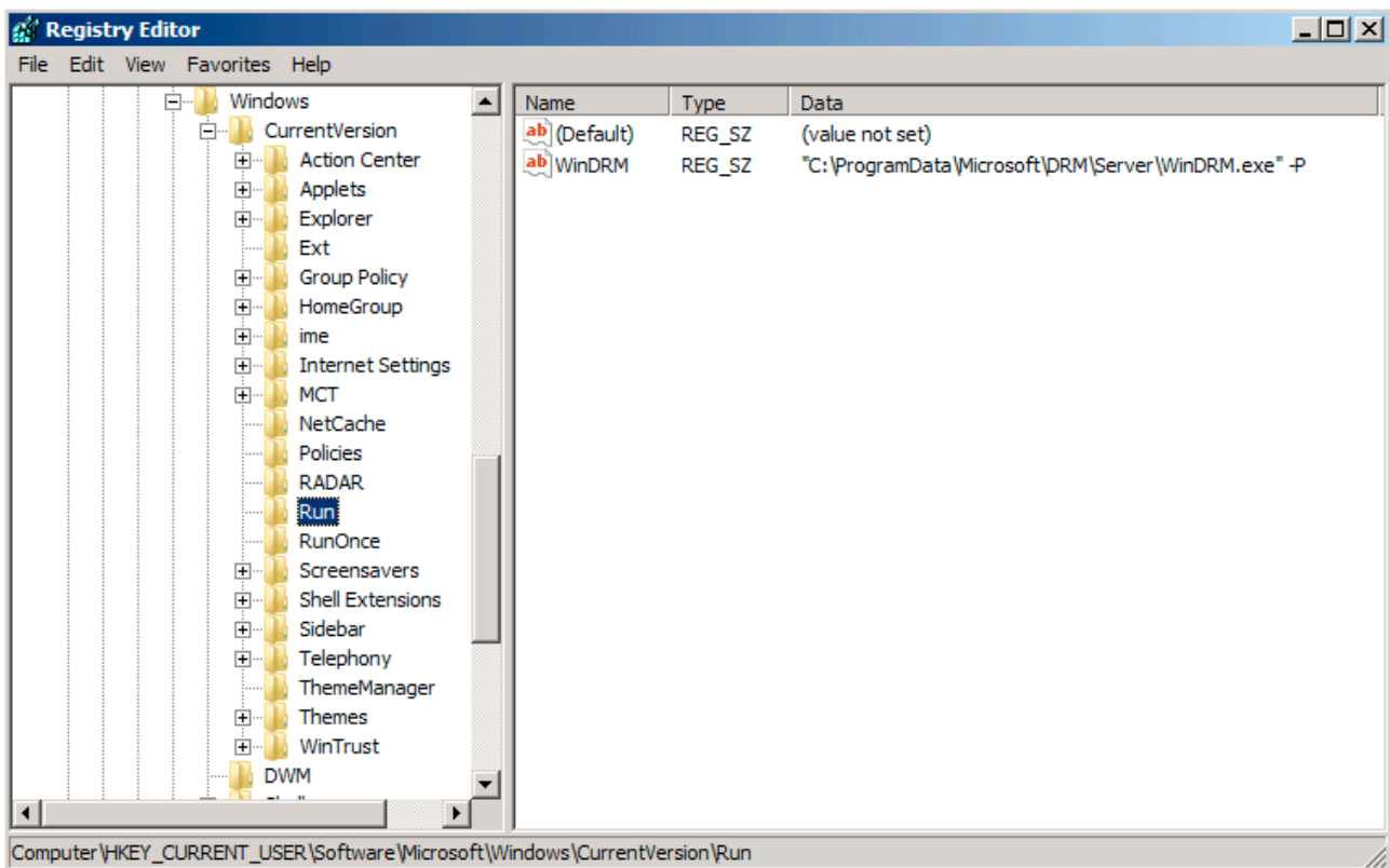
Figure 6. Register as a start program.
