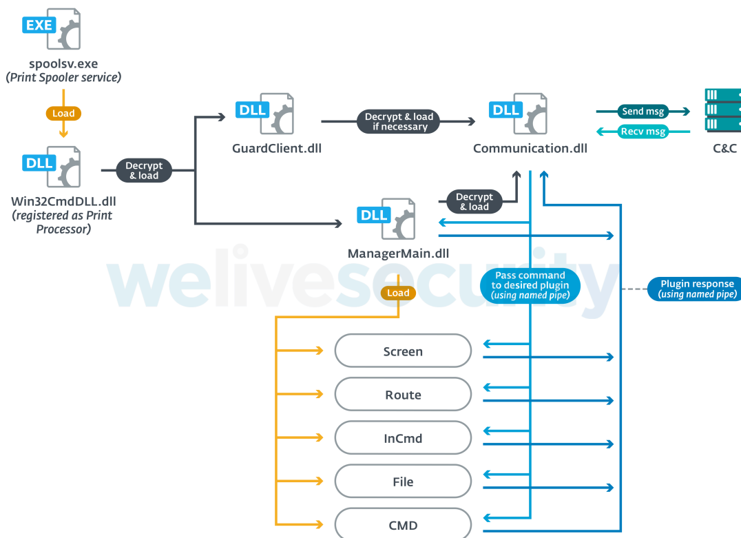
Figure 2. PipeMon IPC scheme (original PipeMon variant)
