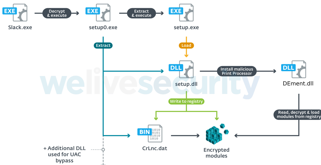
Figure 1. PipeMon staging and persistence
