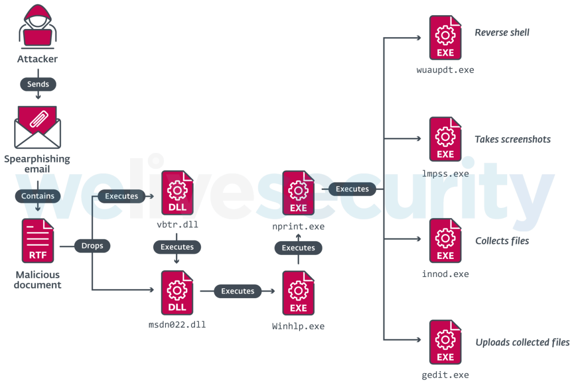
Figure 17. Chain of compromise in Gedit campaigns
