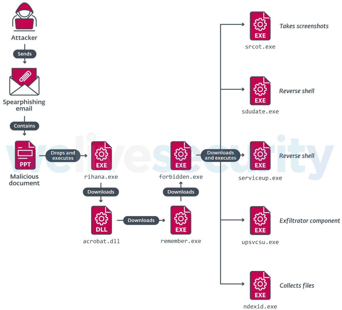
Figure 15. Observed chain of compromise for DarkMusical
