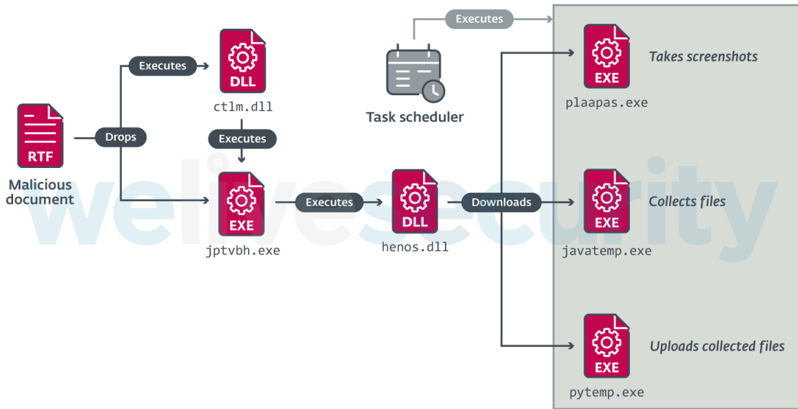
Figure 18. Chain of compromise of the Henos campaign
