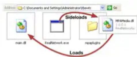
Figure 6 Overview of DLL sideloading process
