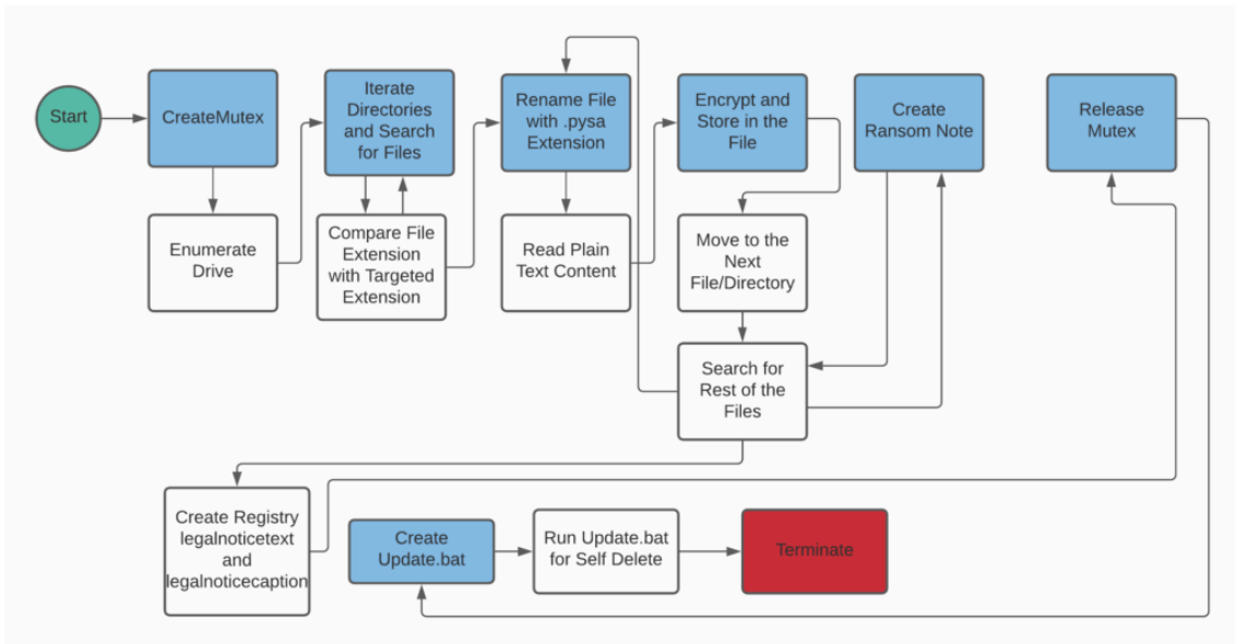
Figure 3 High-level Execution Flow of Pysa Ransomware
