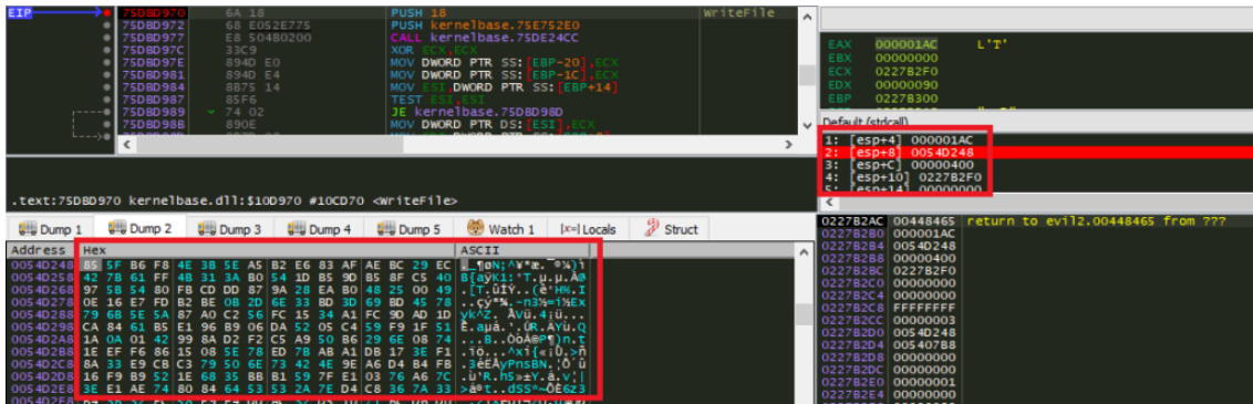
Figure 14 Write Encrypted Content into the File
