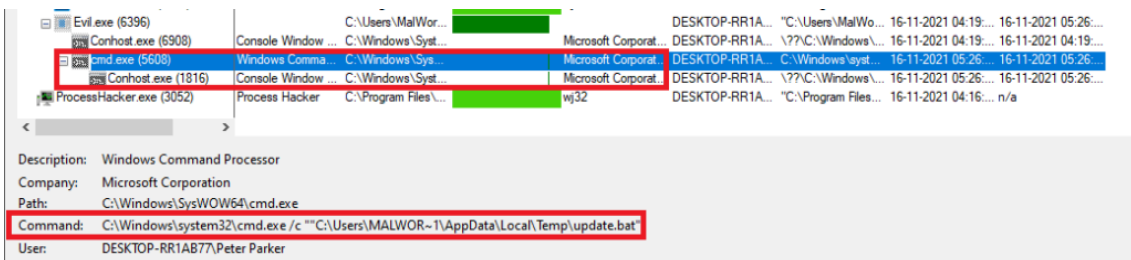
Figure 5 Process Tree
