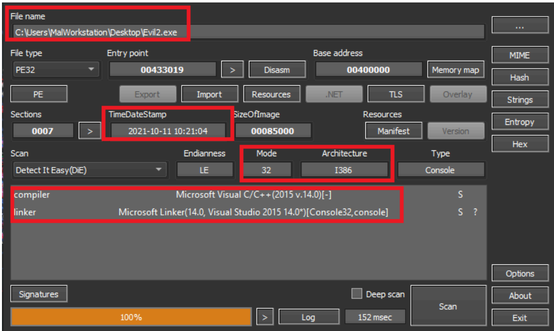
Figure 4 Static Information of Pysa
