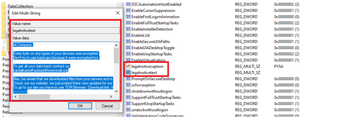
Figure 16 Creates registry legalnoticetext
