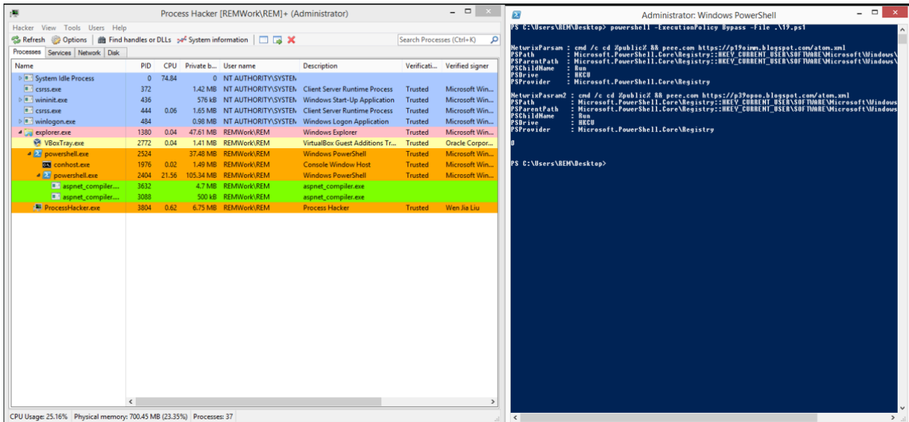
Figure 10. On the left, the PowerShell script can be seen to be launching aspnet_compiler.exe
