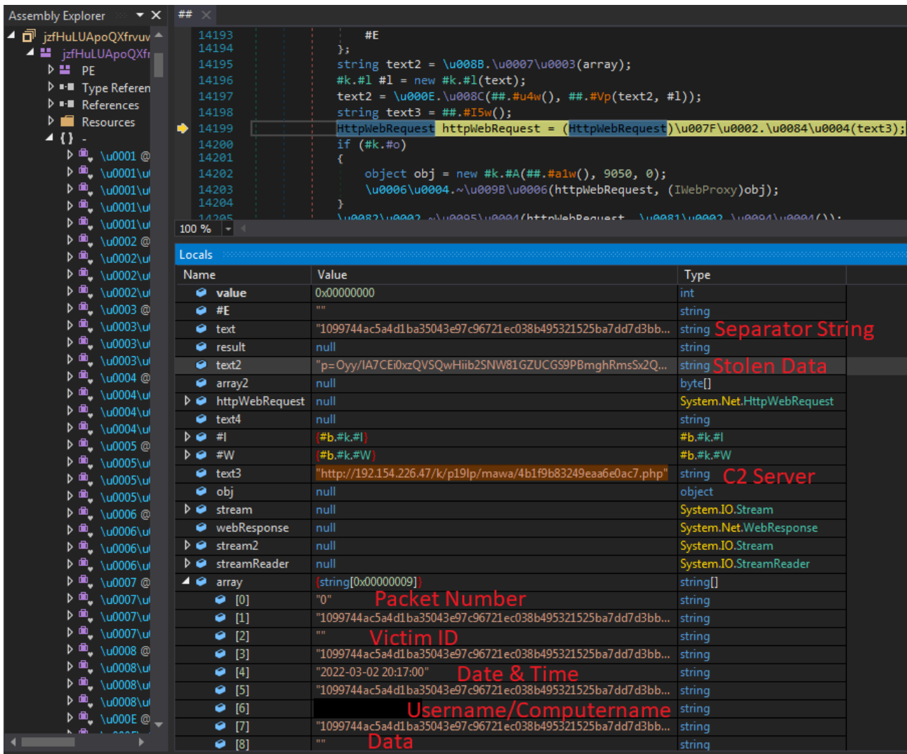
Figure 11. Agent Tesla running inside a debugger.
