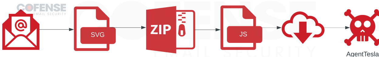
Figure 7: Infection chain of Agent Tesla Keylogger campaign.
