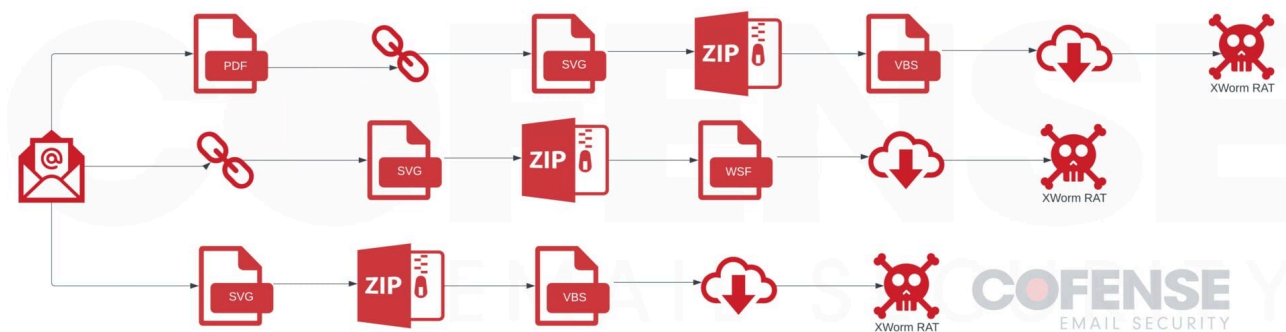
Figure 10: Infection chain of XWorm RAT campaigns.
