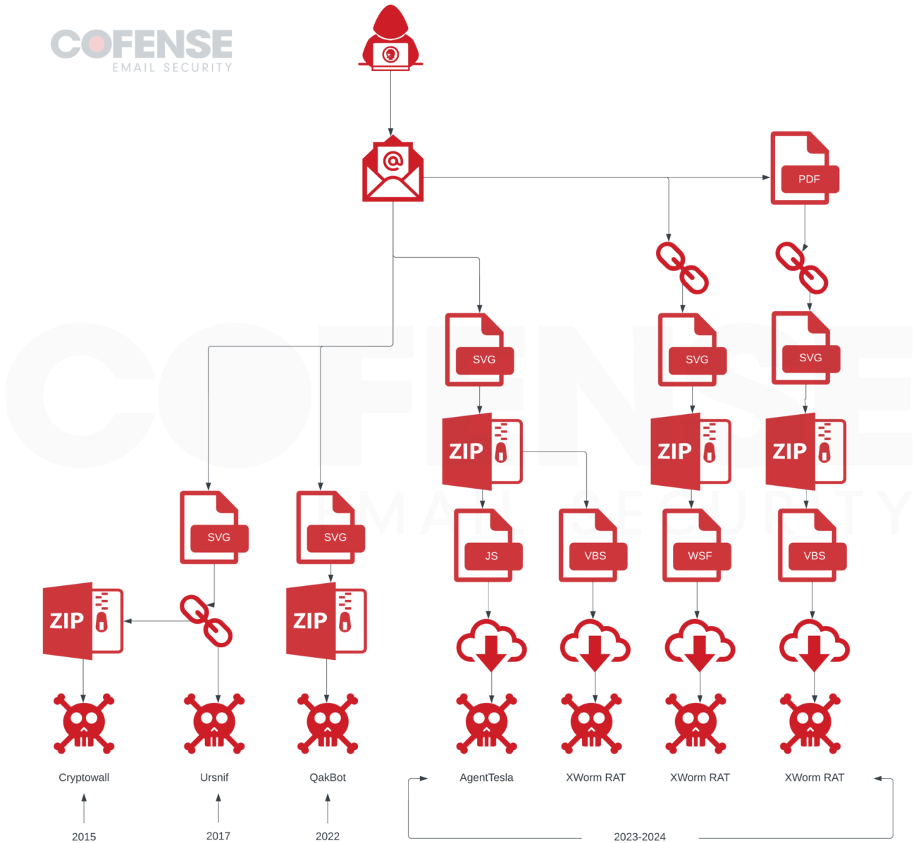
Figure 1: Infection chain of notable SVG file delivery campaigns.
