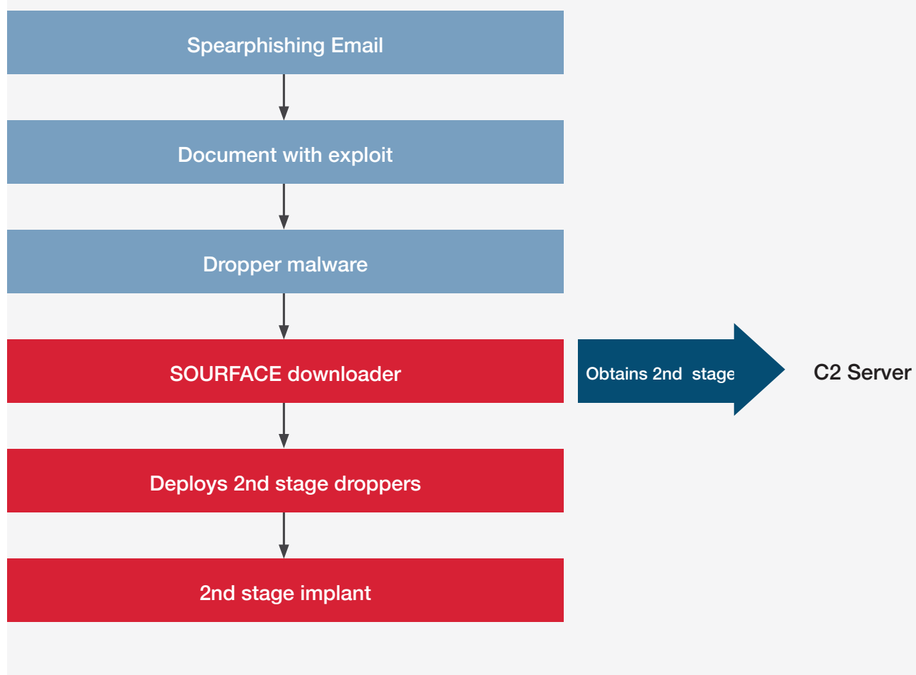
Figure 6: Typical deployment of SOURFACE ecosystem
