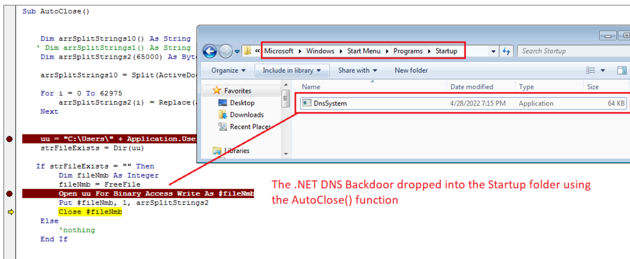
Fig 4. DNS Backdoor dropped in the Startup folder
