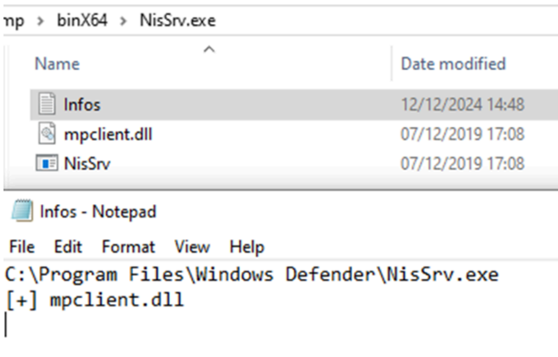
Figure 21. Qualified candidate output
