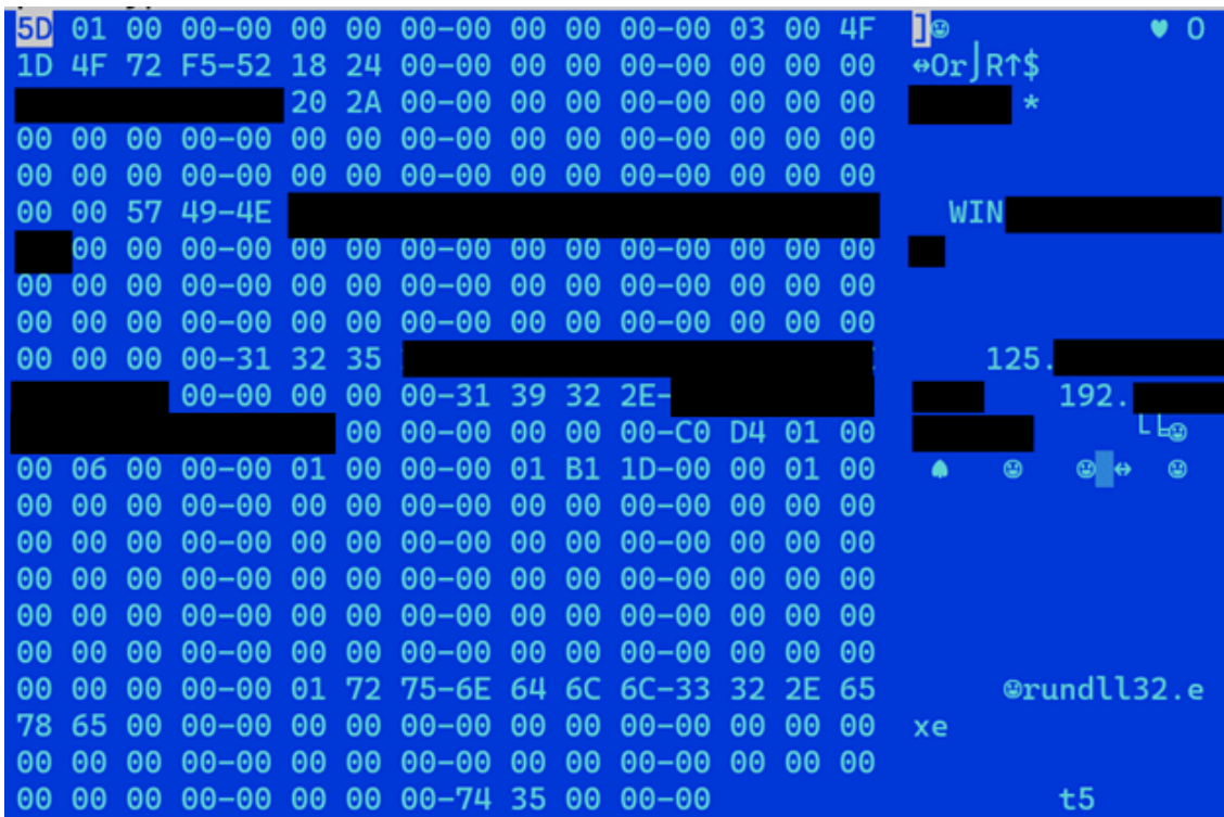
Figure 15. Decrypted data from the backdoor
