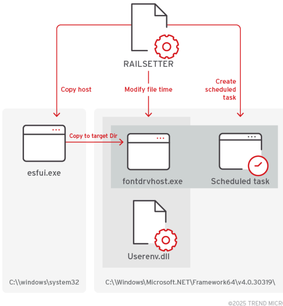
Figure 8. RAILSETTER execution flow
