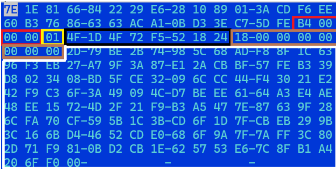
Figure 14. Decoded message from the backdoor
