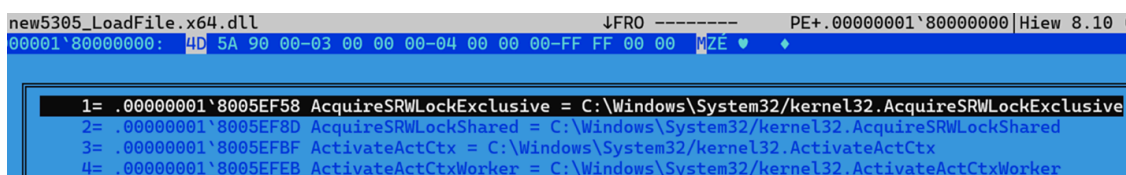
Figure 23. Example of resulting export table
