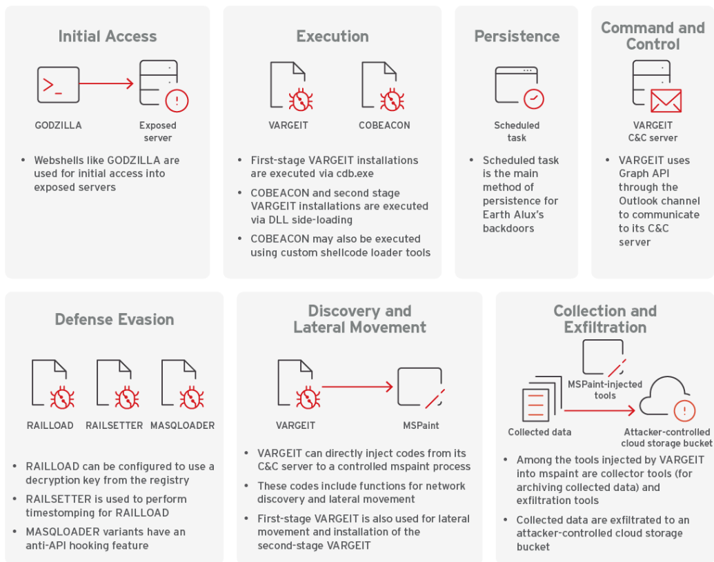
Figure 1. Overview of Earth Alux
