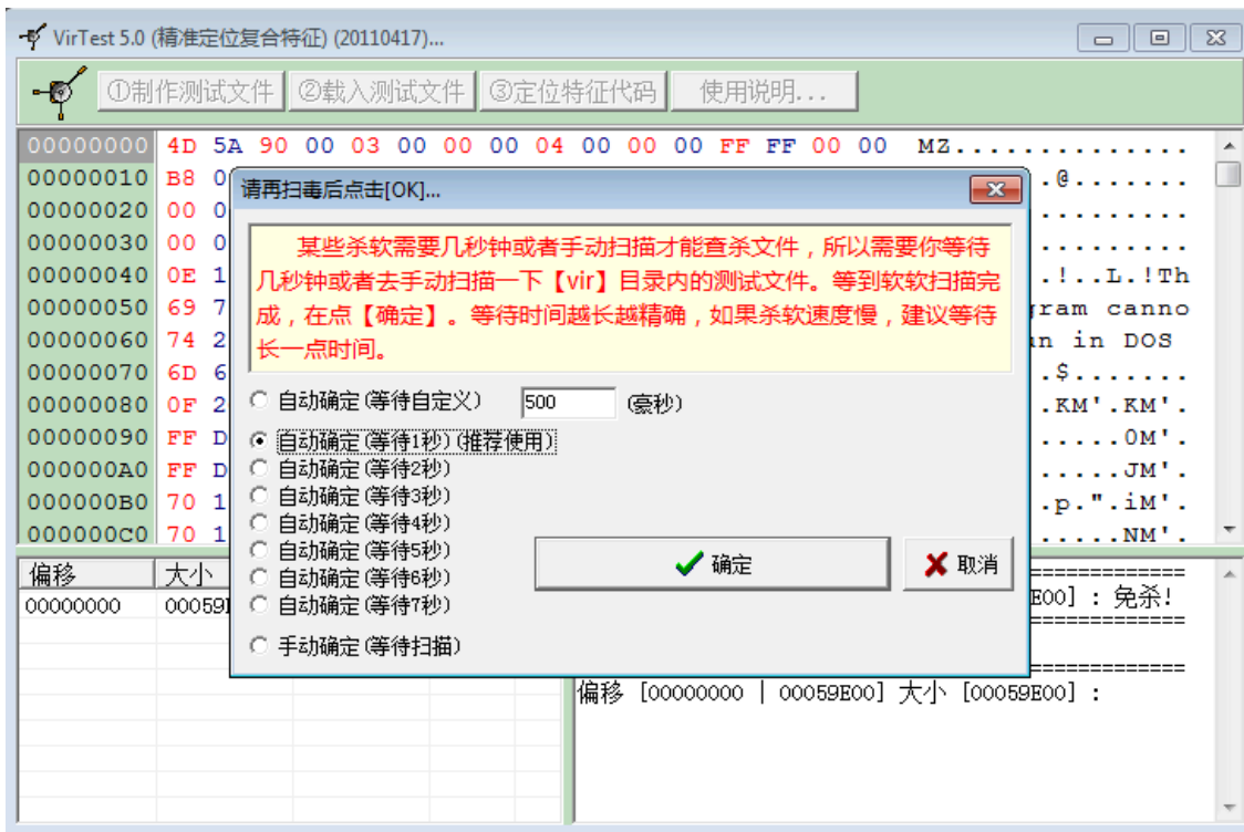
Figure 24. VirTest tool
