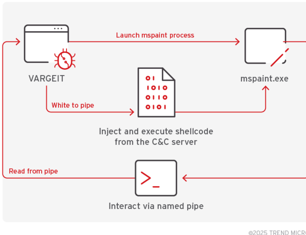
Figure 18. Method 3: Interacting with the injected process via named pipe
