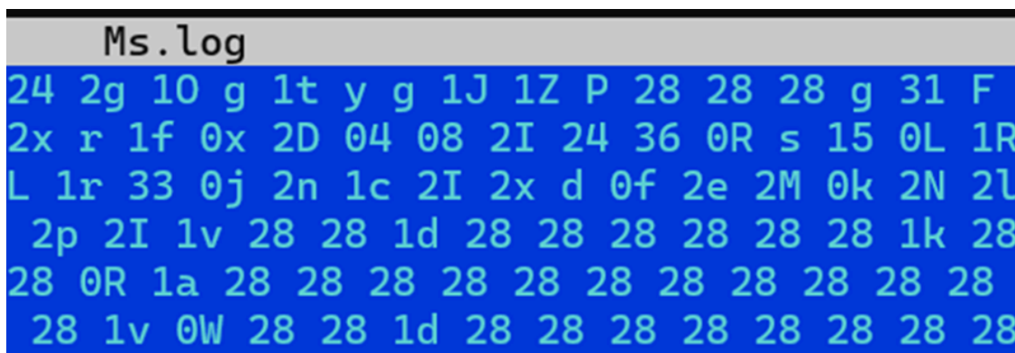
Figure 3. Encrypted payload
