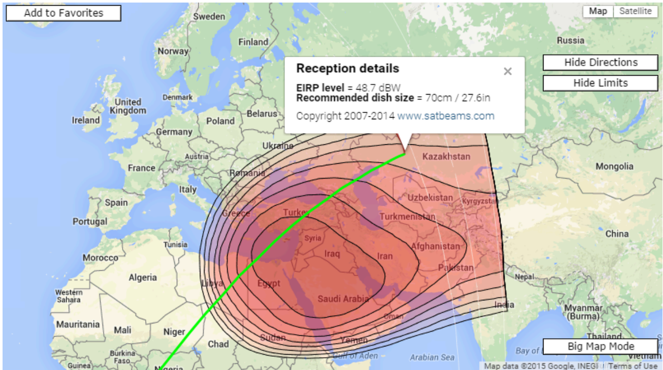
Sample dish calculation – (c) www.satbeams.com
