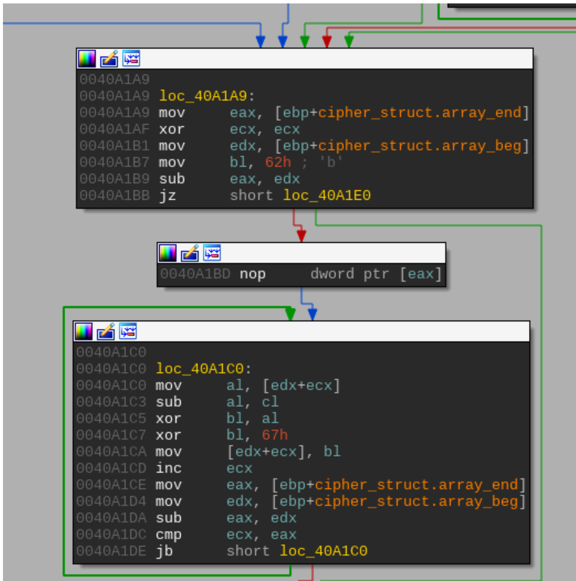
Figure 5. Phase Three of the decryption process
