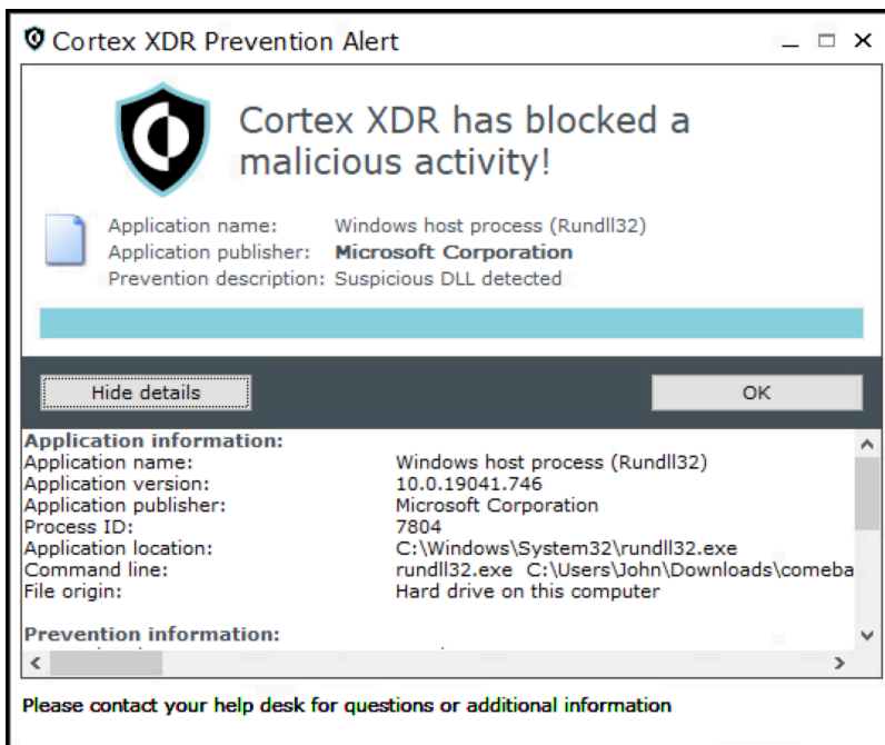
Figure 15. Alert from Cortex XDR blocking Comebacker malware.
