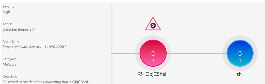
Figure 9. Cortex XDR alert detecting ObjCShellz activity.
