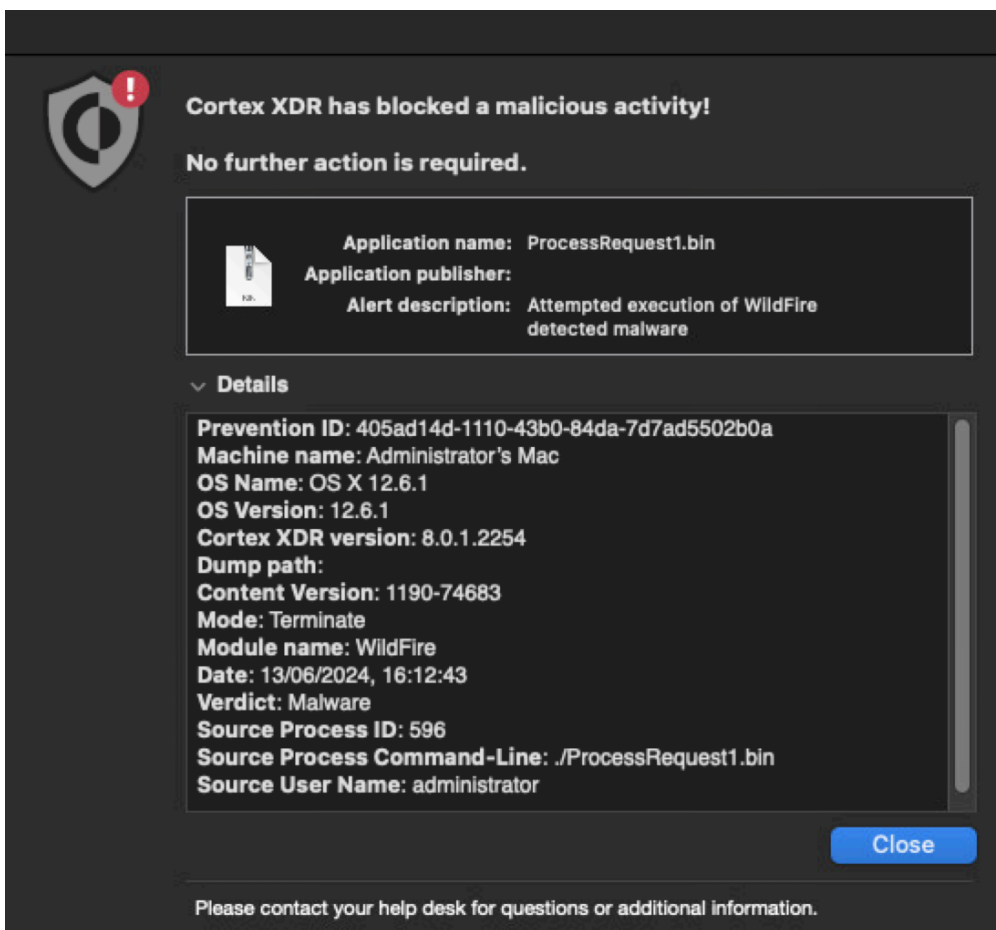
Figure 11. Fullhouse malware prevented by Cortex XDR.
