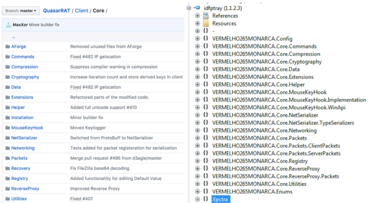
Figure 2—Similarity between Quasar RAT and XPCTRA directory trees
