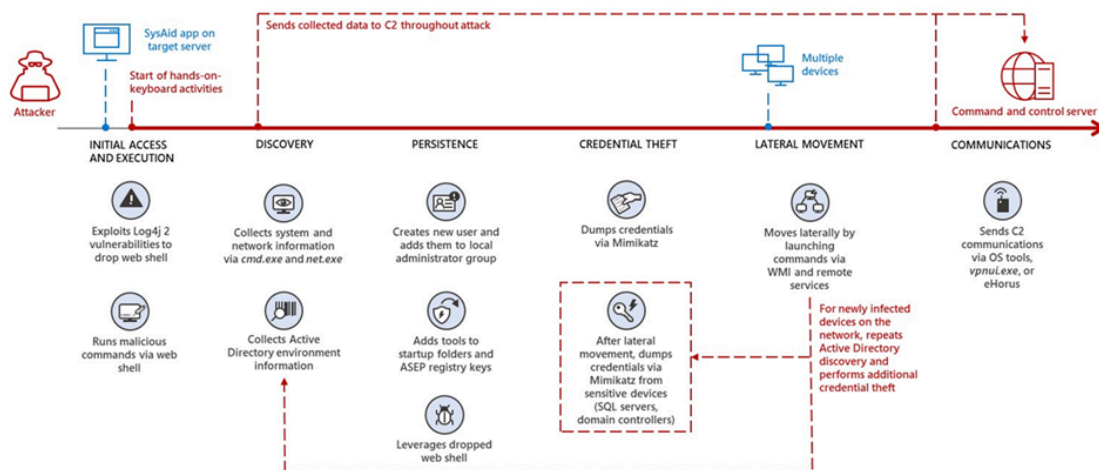
Figure 1. Observed MERCURY attack chain
