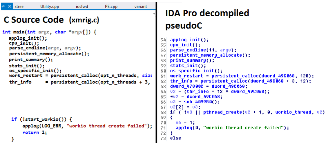
Figure2. Code comparison between original and adapted versions
