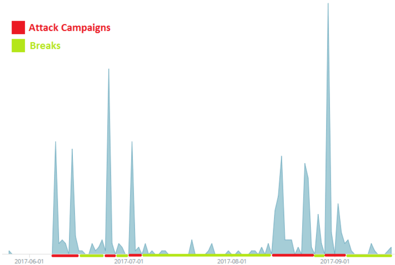
Figure4. Graph of infection waves over time
