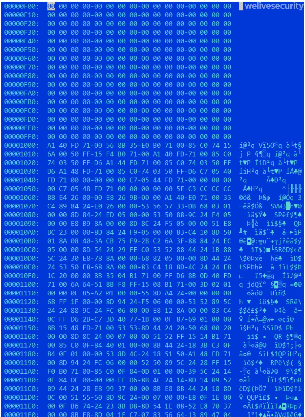
Figure 3. The PE header is missing in the newly built backdoor from the MpSvc.dll shellcode
