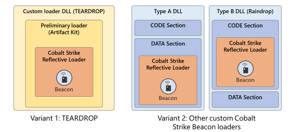
Figure 4. Structure of the two variants of Cobalt Strike Beacon loaders observed in Solorigate attacks
