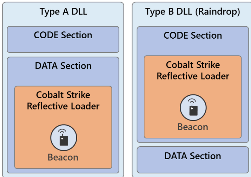
Figure 9. Two subtypes of the custom Loader
