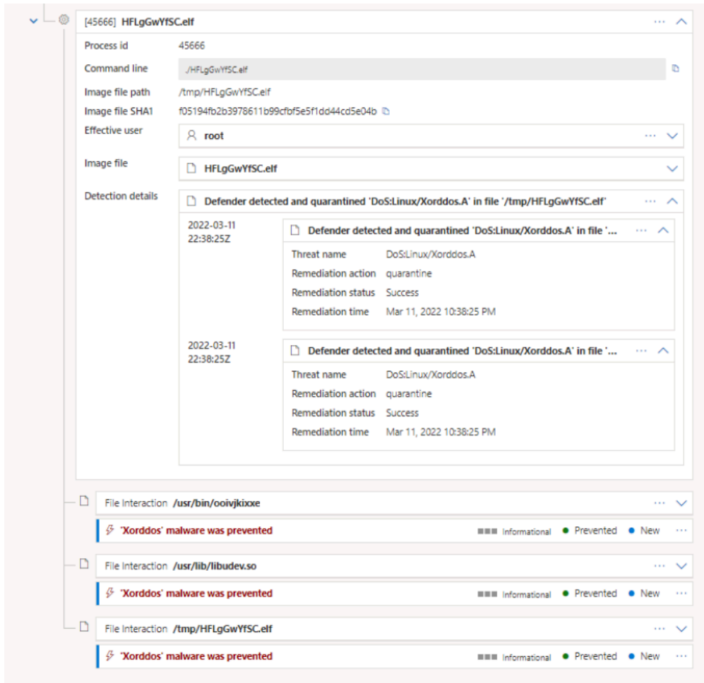
Figure 24. Microsoft 365 Defender alert for detection of XorDdos malware
