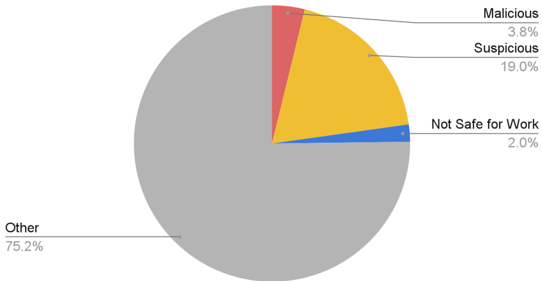
Figure 3. Category distribution of strategically aged domains.
