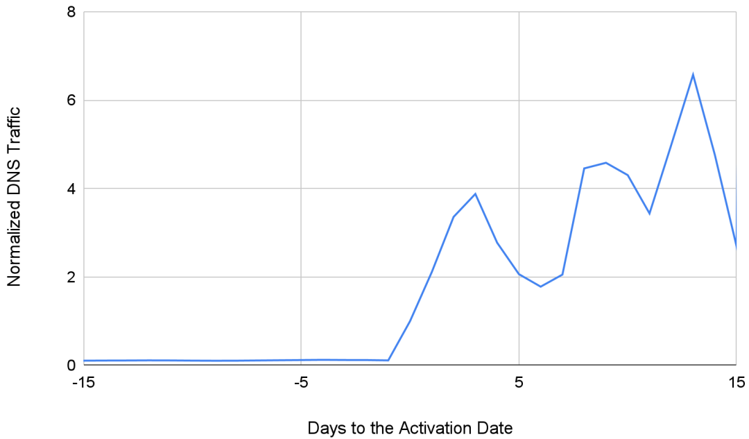
Figure 2. Normalized DNS traffic of strategically aged domains.
