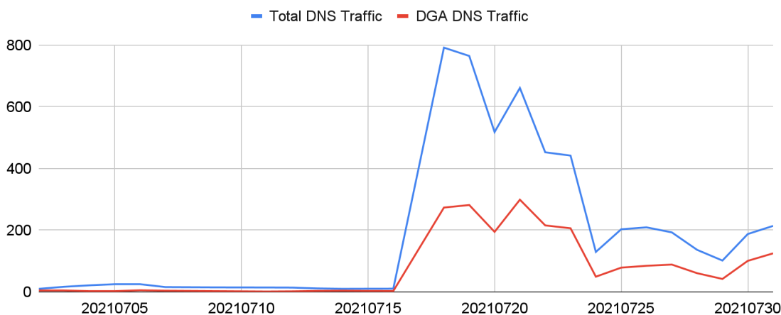
Figure 5. DNS traffic trend of Pegasus spyware C2 domains.
