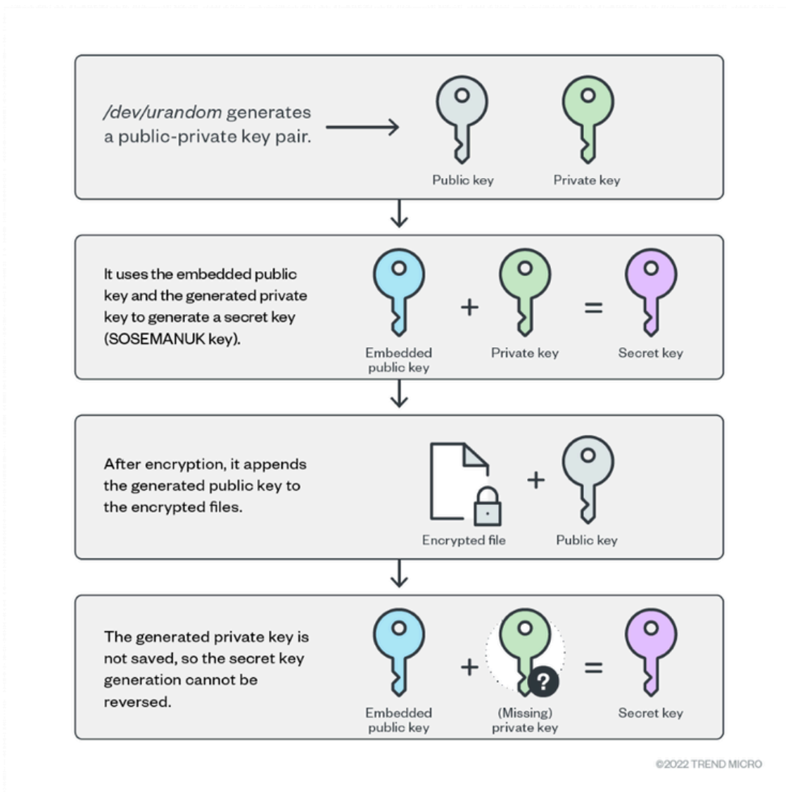
Figure 5. Cheerscrypt’s encryption algorithm
