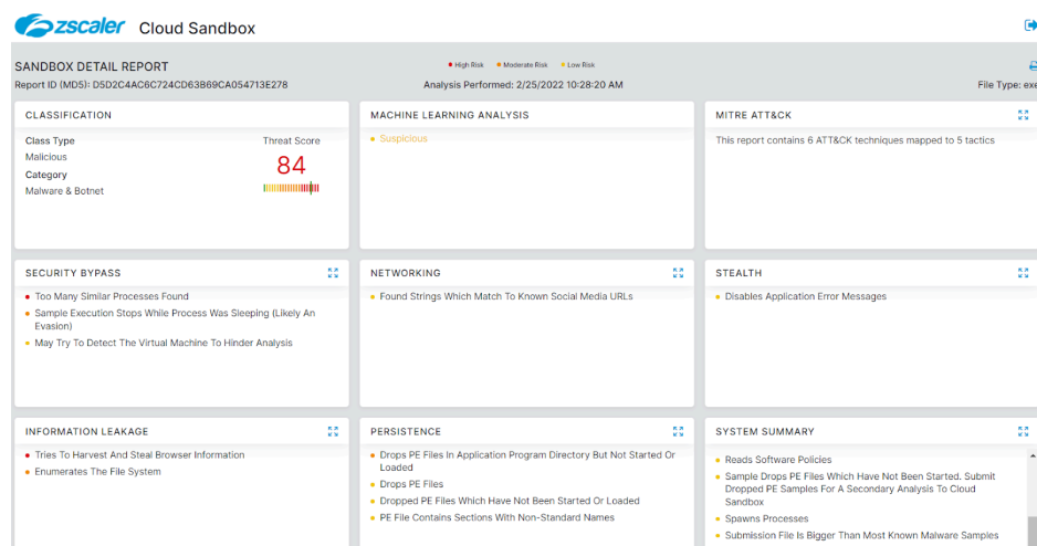
Figure 5. Zscaler Cloud Sandbox Report - PartyTicket
