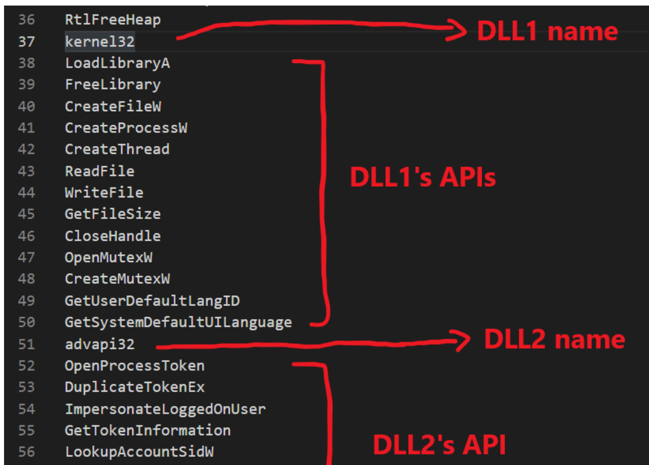
Figure 9: Decrypted library table layout
