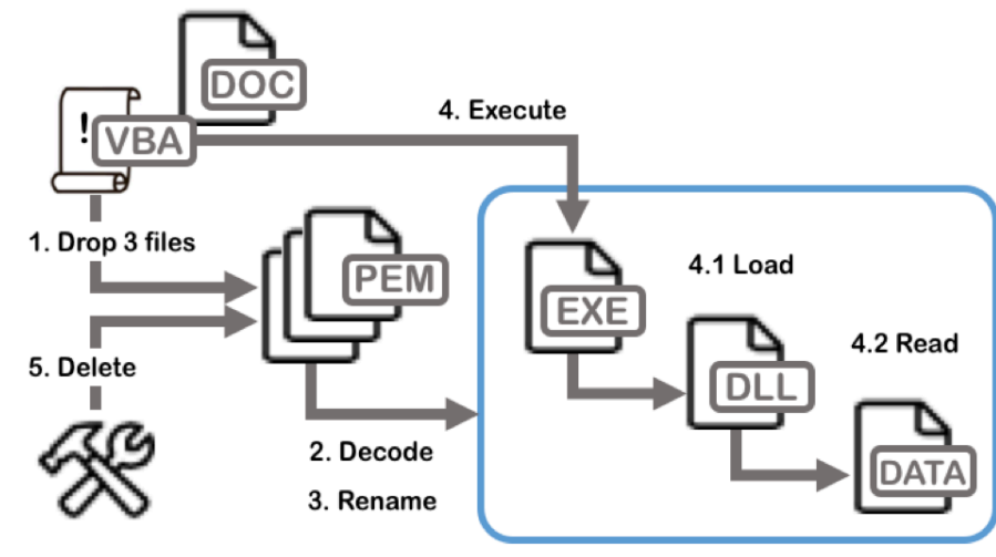
Figure 7: Attack overview
