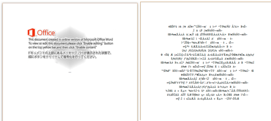
Figure 4 shows what happens when the malicious macro is executed.
