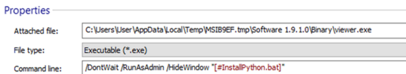
Figure 17. Custom Action script of the latest Batloader campaign observed in Q4 2022
