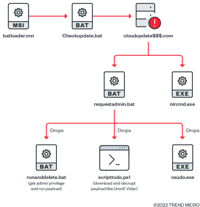
Figure 7. Batloader kill chain using compromised MSI package
