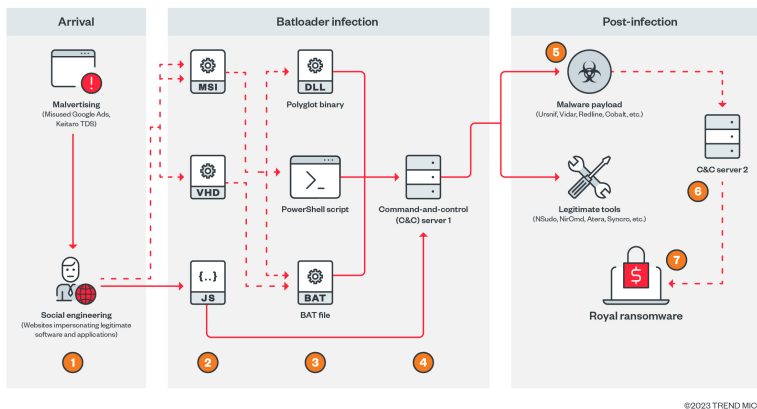
Figure 3. Typical Batloader kill chain
