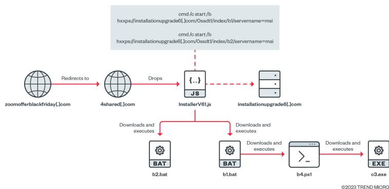
Figure 15. A typical execution chain for the JavaScript Batloader campaign
