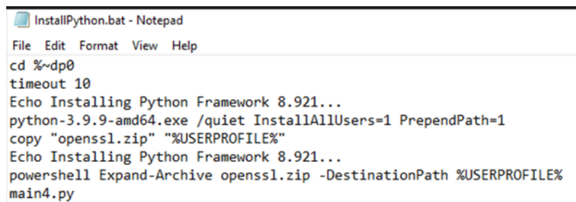
Figure 18. InstallPython.bat
