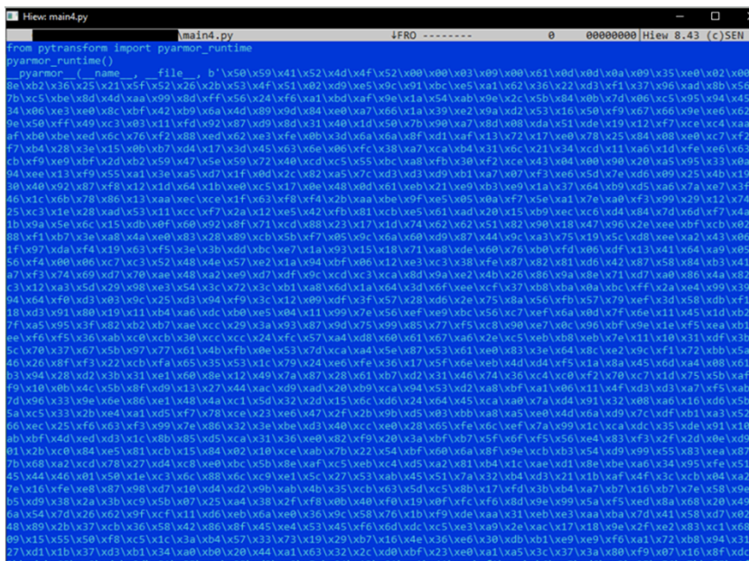
Figure 19. Batloader PyArmor-protected Python script
