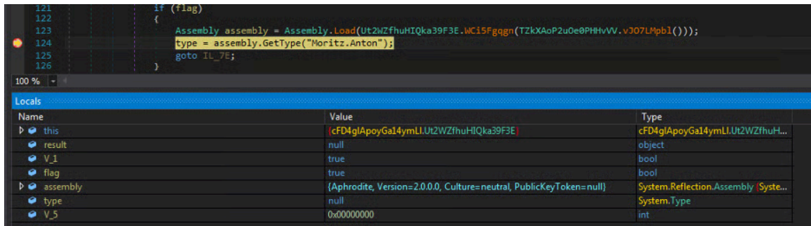
Figure 9: The unpacked and loaded second stage DLL called Aphrodite.
