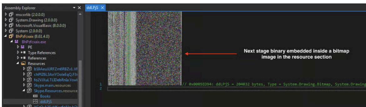
Figure 11: The bitmap image inside the resource section that contains the next stage payload.
