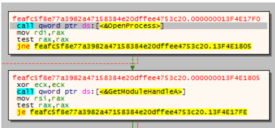
Ryuk getting a handle to the target process.
