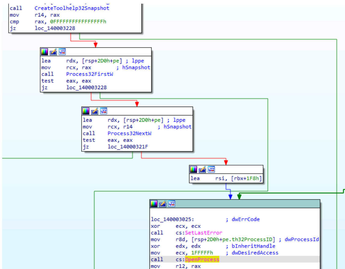
Ryuk enumerating system processes.
