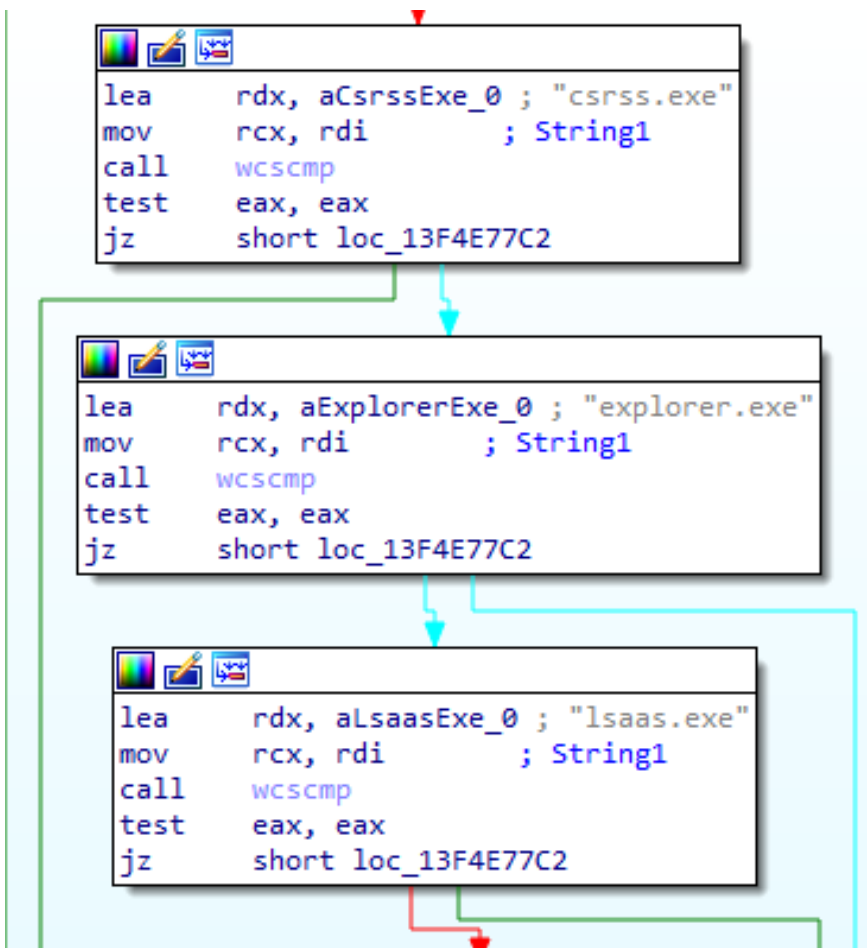
Ryuk process-injection safeguards.
