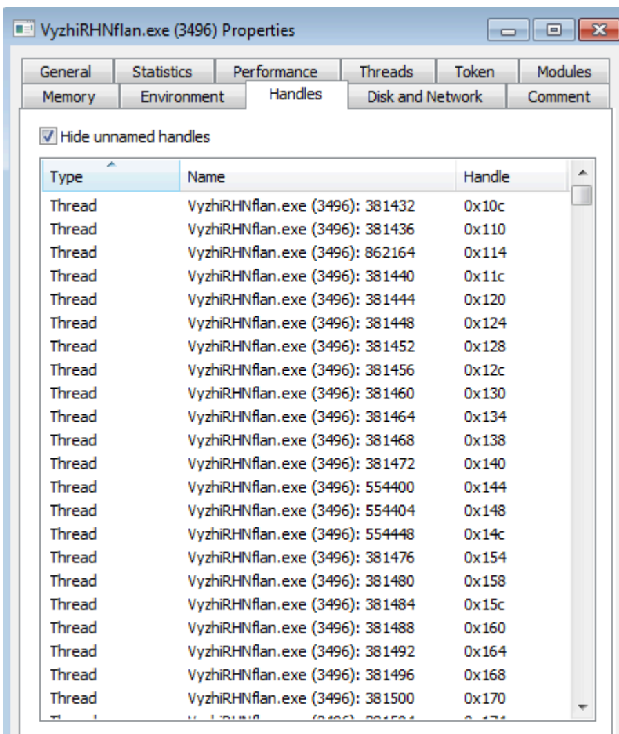
Ryuk encryption threads.
