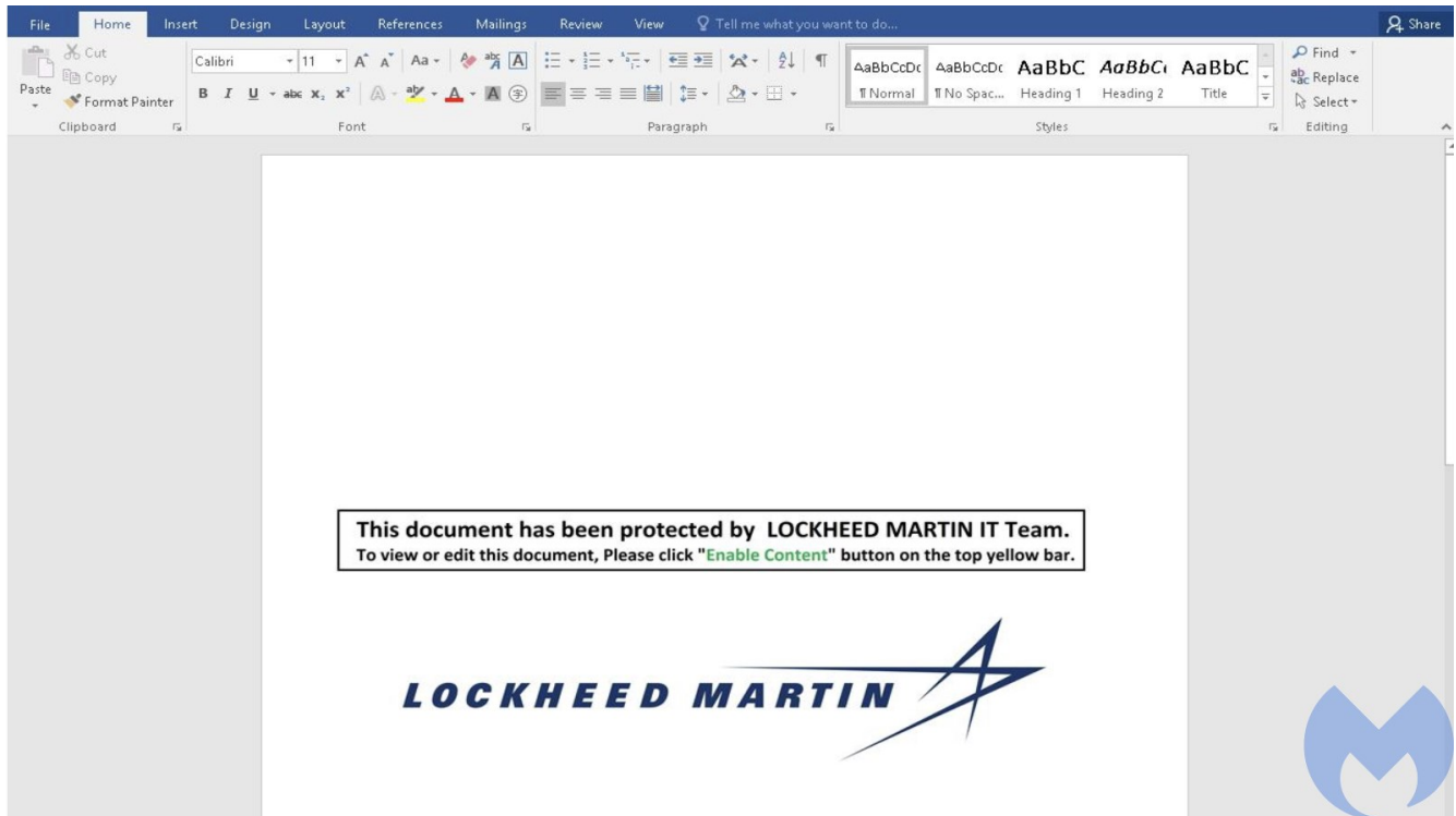
Figure 1: Document Preview
