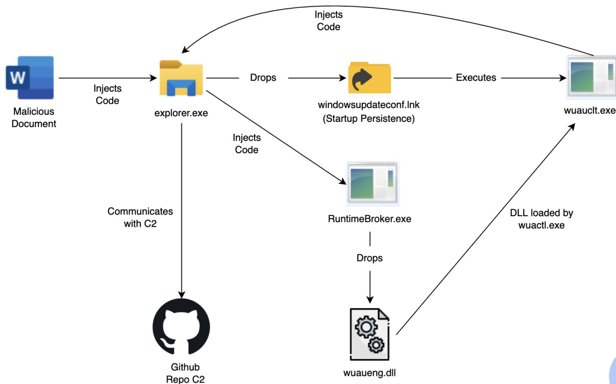
Figure 2: Attack Process
