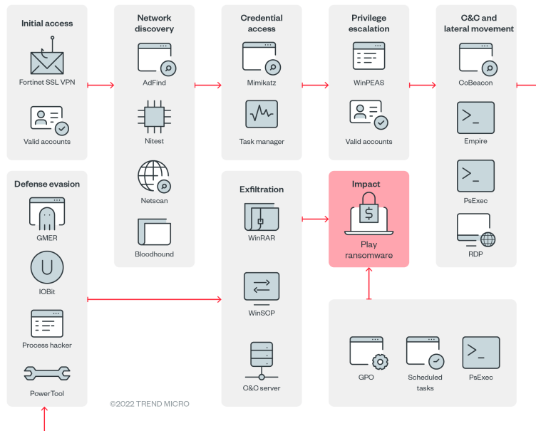
Figure 3. Play ransomware's infection chain
