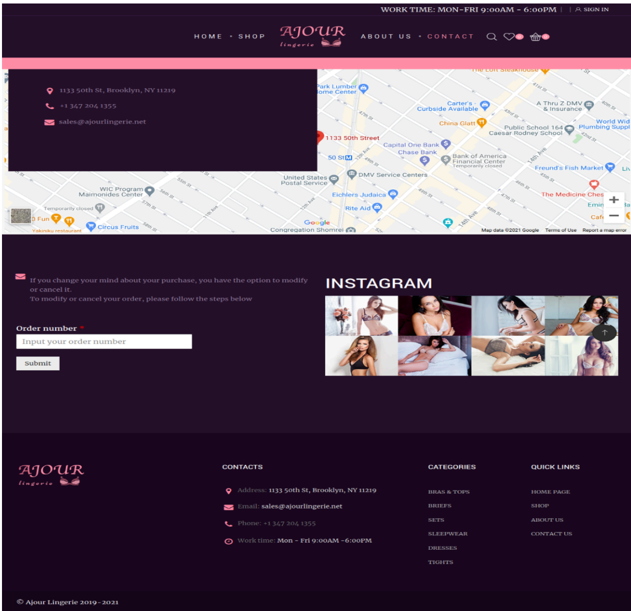
Figure 5: Landing Page
