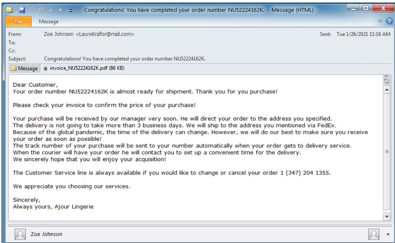
Figure 3: Email Lure
