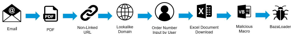
Figure 1: Infection Chain
