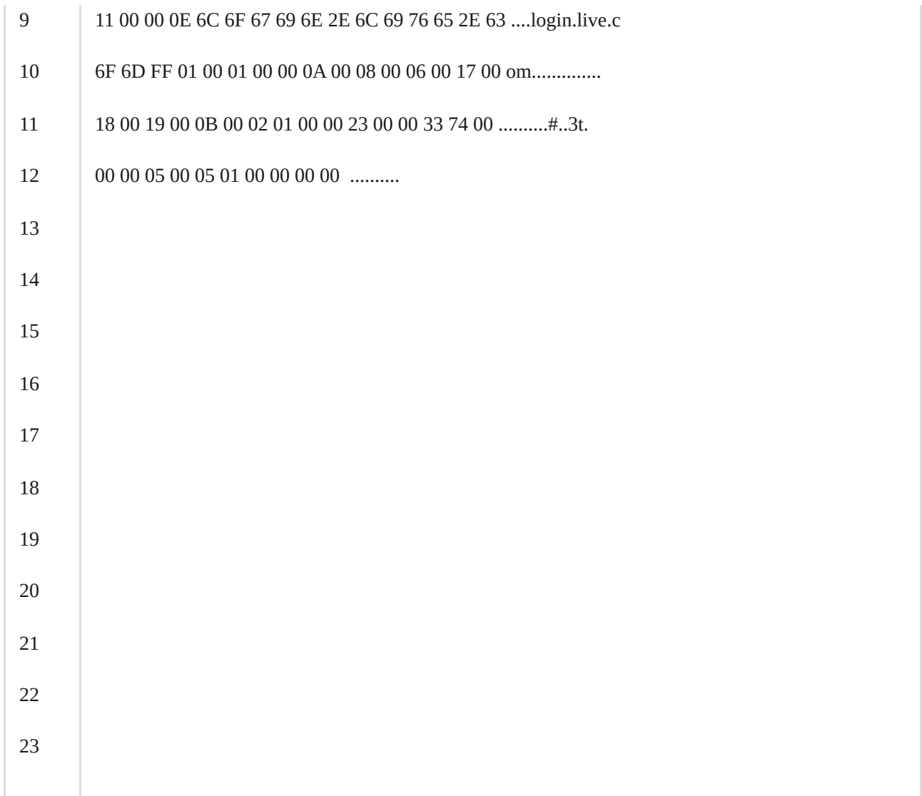
Figure 1. Hardcoded buffer used as the TLS Client Hello packet sent to the C2 server
