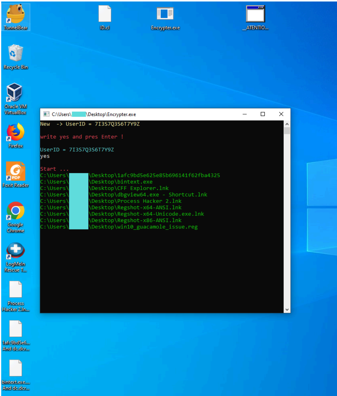
Figure 9: Ransomware execution
