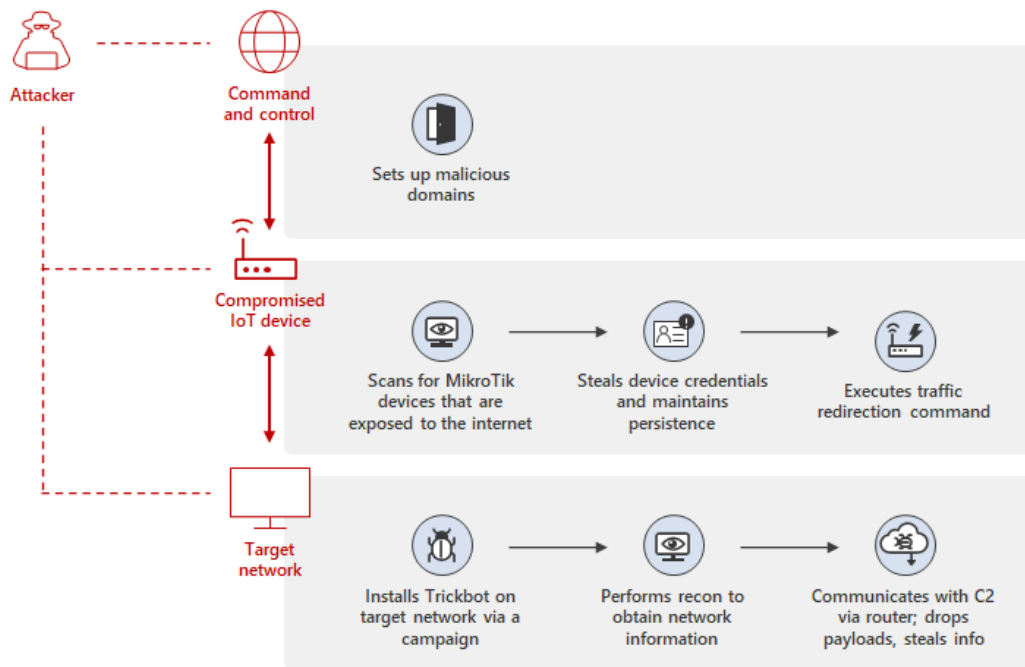
Figure 1. Trickbot attack diagram
