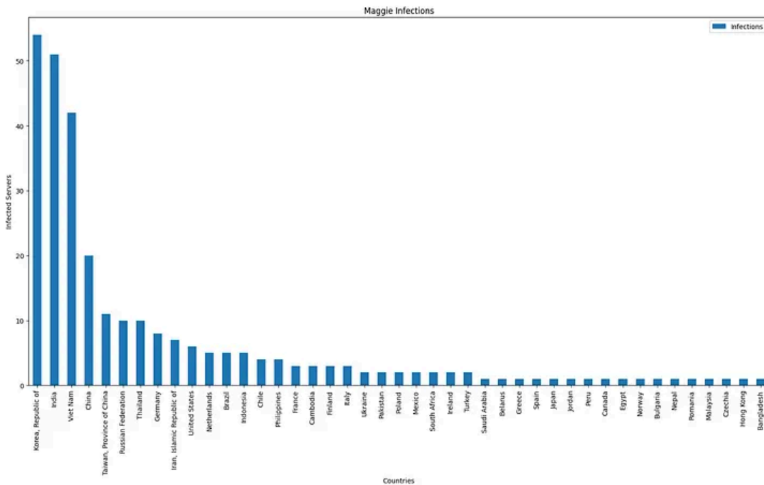
Prevalence of backdoor user by country
