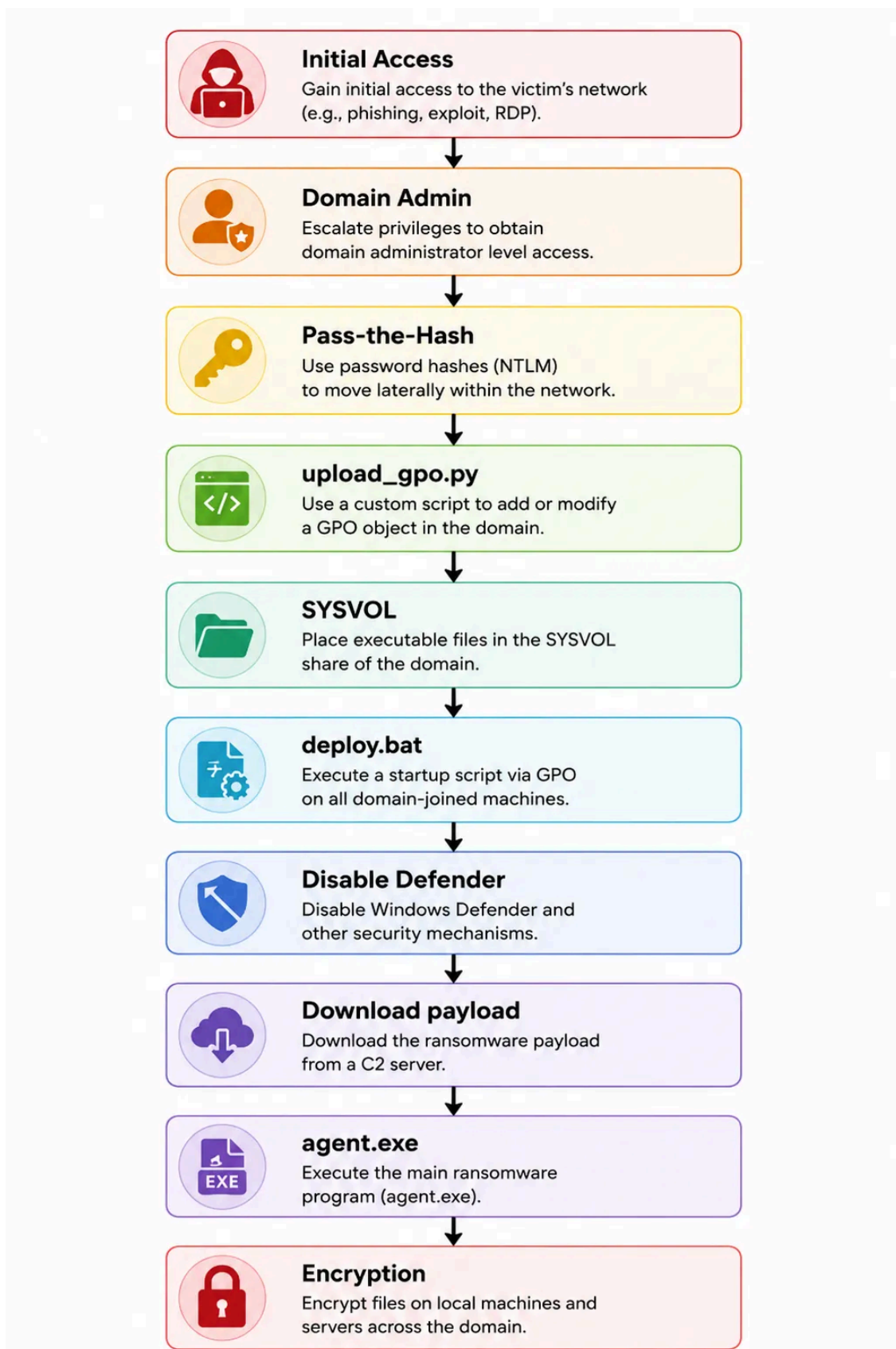
Figure 10. INC Ransom attack chain based on the identified tools.
