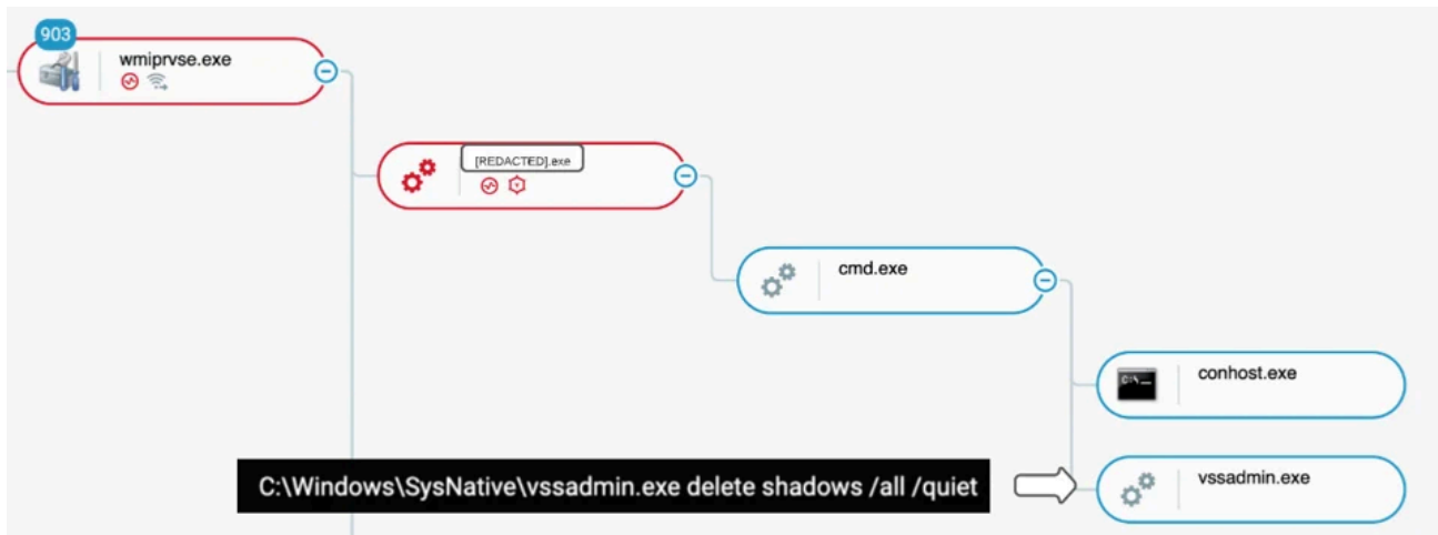
Cybereason process tree showing [REDACTED].exe launching cmd.exe which calls vssadmin.exe
