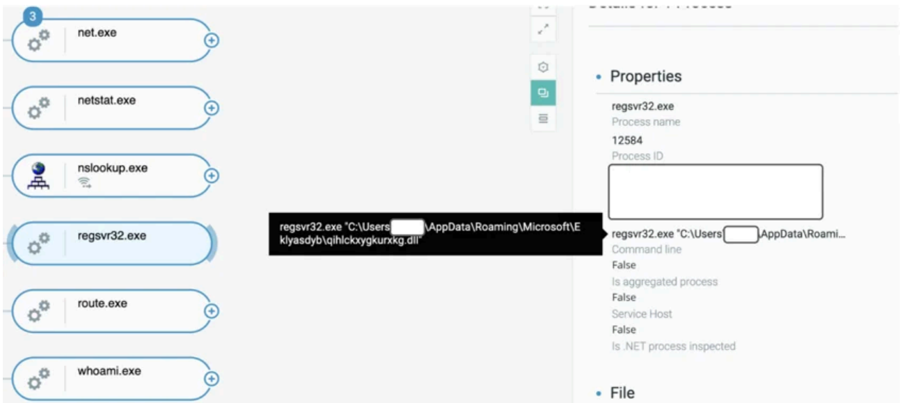
Regsvr32.exe trying to load a DLL
