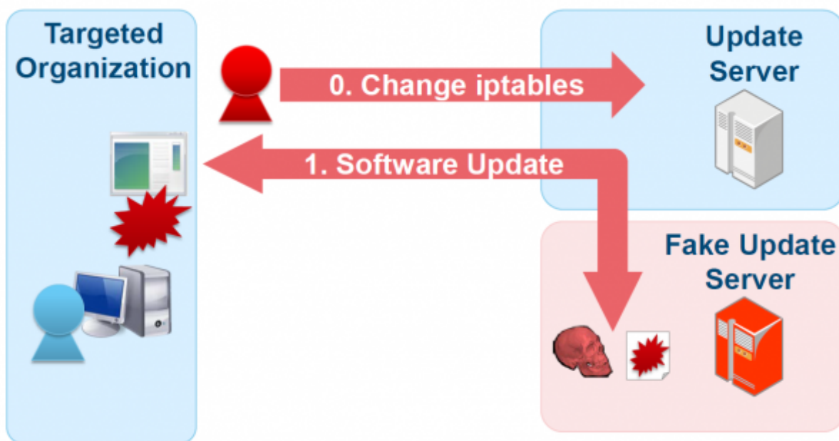
23: Update hijacking.
