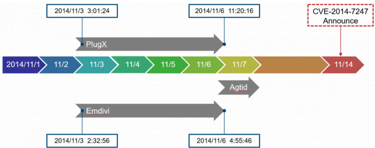
Figure 8: Timeline.
