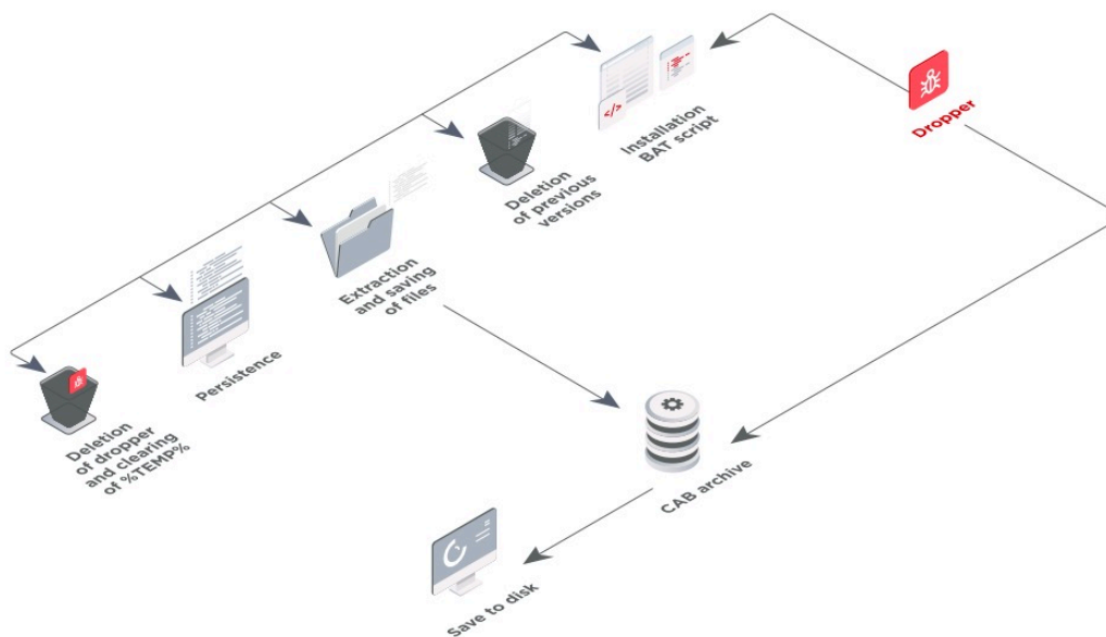
Figure 9. Malware structure and installation process
