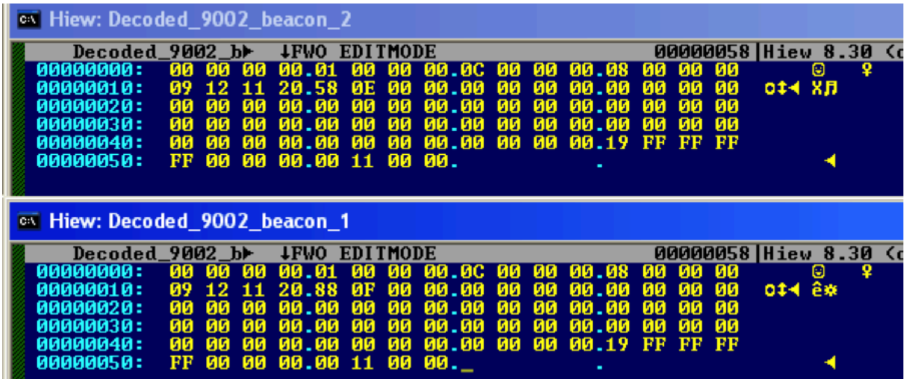
Figure 8 - XOR decrypted callback beacons of the diskless 9002 RAT payload
