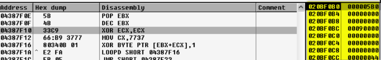
Figure 2 – Shellcode launches rundll32.exe and injects payload
