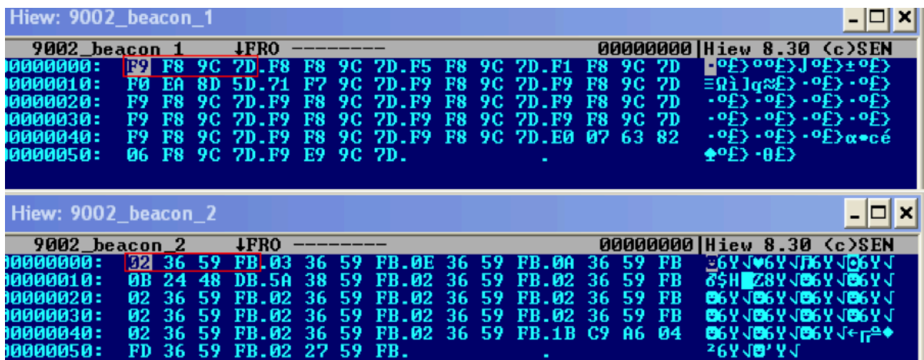
Figure 7 - Sample callback beacons of the diskless 9002 RAT payload
