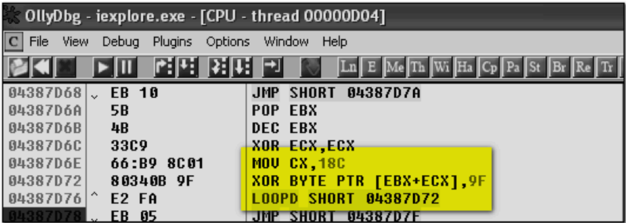
Figure 1 - Initial XOR decoding of shellcode, with key '0x9F'
