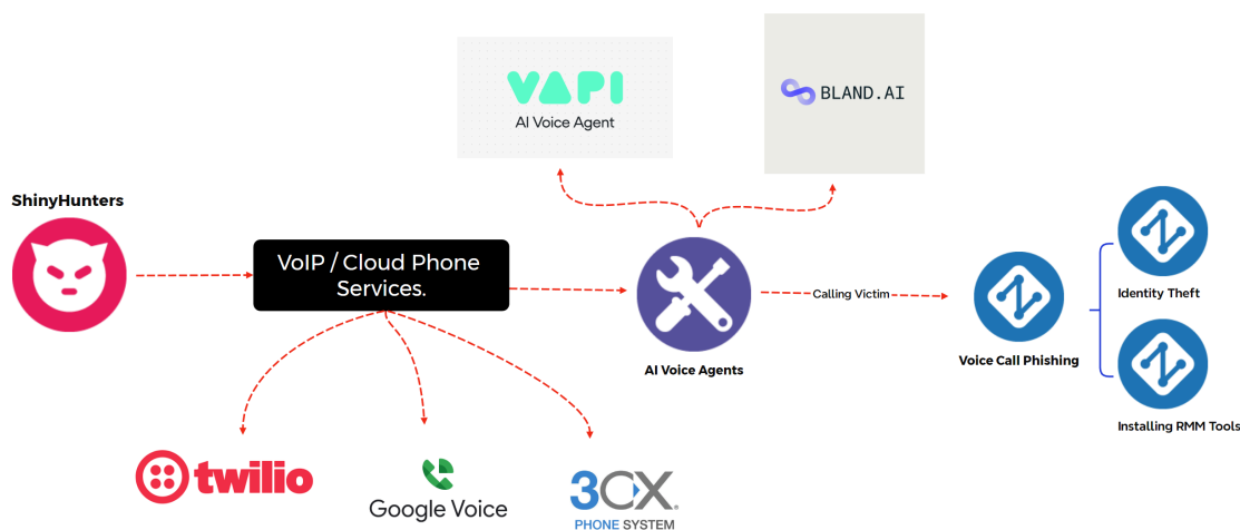
Figure 4 - AI Voice Agent workflow in Vishing campaigns.
