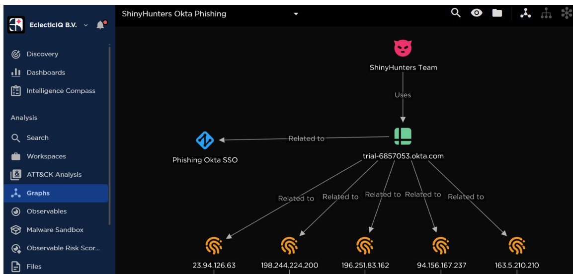
Figure 13 - Link analysis of the Phishing infrastructure in EclecticIQ's TIP.
